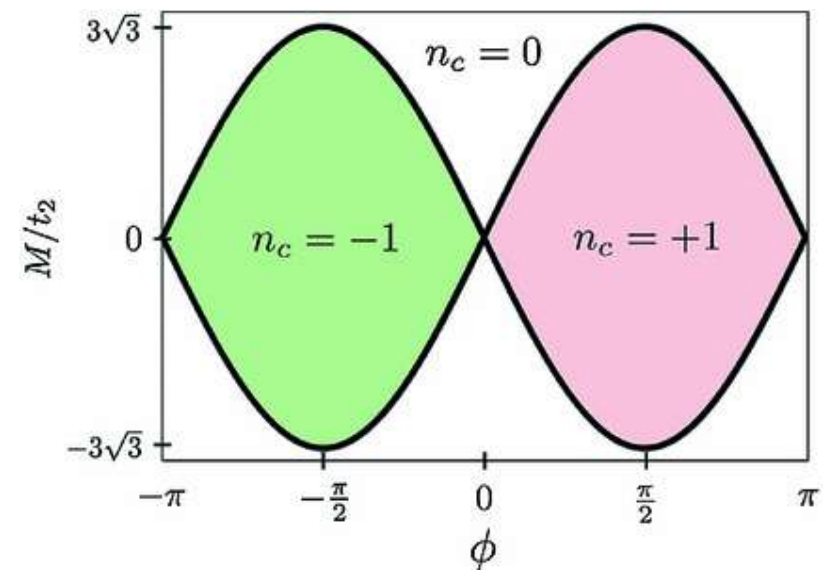
Haldane model phase diagram
