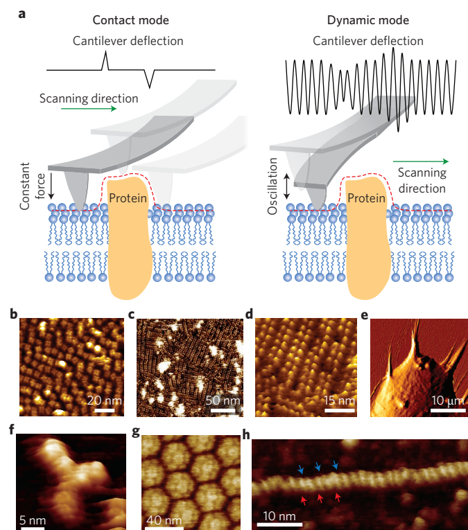
Figure 2 | AFM-based imaging of native biological systems to molecular resolution.
