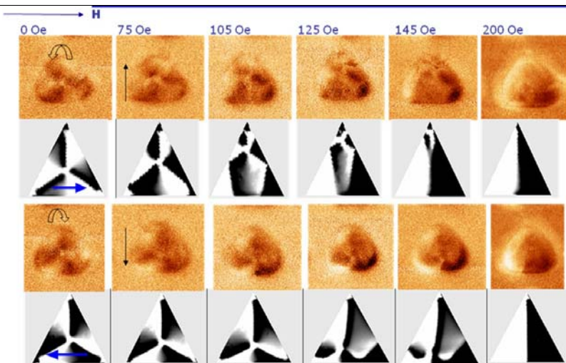
Figure 8. High-resolution VFMFM images and results of micromagnetic simulation for the magnetization process of a vortex state in triangular nanodots. (Phys.Rev. B 81 (5), 054439 (2010))
