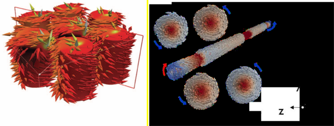
FIGURE 5. Images of micromagnetic simulations of the magnetization distribution at the remanence state for arrays of seven Co nanopillars with diameter of 75 nm (Y. Ivanov et al. Nanotechnology 24 (2013) 475703), and of an individual CoFe nanowire with modulations in diameter (J.A. Fernandez-Roldan, submitted)
