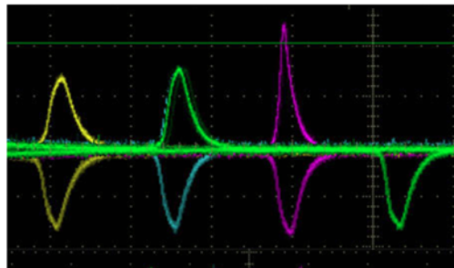
FIGURE 1- Sequences of induced signals at the pickup coils along a bistable microwire where the collapse of two domain walls propagating in opposite directions is detected. (A. Jimenez et al. Eur Phys J B 86 (2013) 113)
