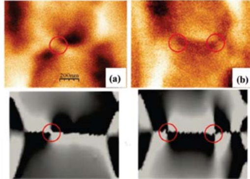
FIGURE 6. High-resolution MFM images (up) and results of micromagnetic simulation (down) for vortex (a) and double vortex (b) DWs in a Cobalt nanostripe. (Phys.Rev. B 87, 184410 (2013))
