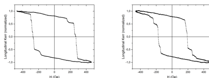
MOKE local hysteresis loops at different positions along a multisegmented FM/Metal individual nanowire denoting the propagation of a domain wall
