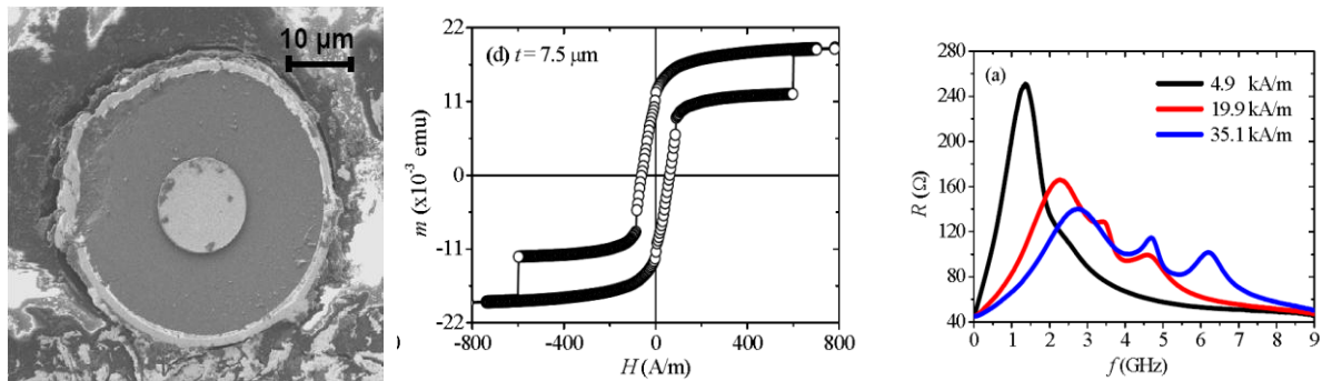
FeSiB/CoNi bimagnetic microwire (left); hysteresis loop of a soft/ultrasoft FeSiB/NiFe bimagnetic wire (center) and the impedance spectrum with static field as the parameter for a CoFeSiB/NiFe microwire (right) (G. Infante PhD, 2010)
