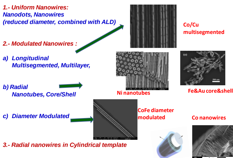
Different families of nanowires with cylindrical symmetry investigated
