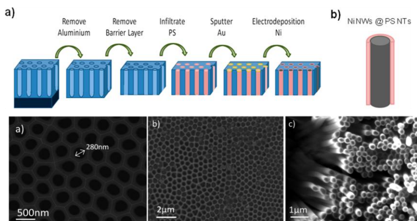
Top view SEM images of AAO membrane with average pore diameter of 280 nm and interdistance between pores of 420 nm (a), polystyrene nanotubes embedded into AAO membrane (b), and polystyrene nanotubes out of AAO membrane (c).
