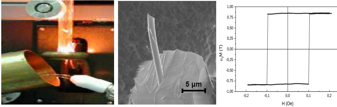
Glass-coating cast unit during the quenching fabrication (left); FeSiB glass-coated (center) and its bistable loop (right)
