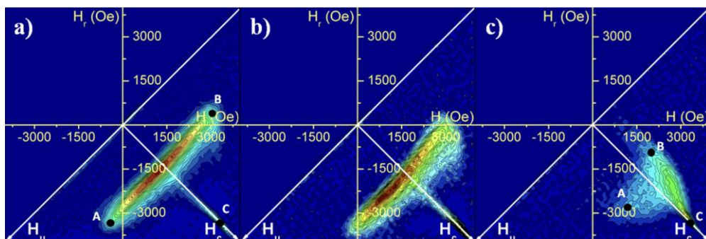
FORC distributions for FeCo/Cu multilayer nanowire arrays as a function of the Cu layer thicknesses for the same FeCo segment thickness [(\text{FeCoCu} (300 \text{ nm}) / \text{Cu}(x))_{10}] : (a) x=7 \text{ nm} , (b) x=15 \text{ nm} and (c) x=40 \text{ nm} (E. Palmero et al. Nanotechnology 27 (2016) 435705).
