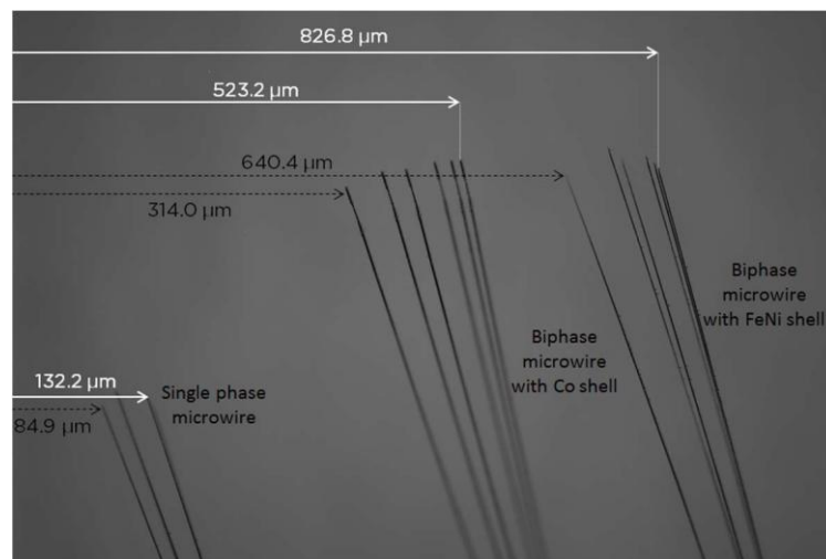
Micro-actuator based on bimagnetic core/shell microwires with asymmetric external shell (Patented, 2017). Image showing the bending under increasing applied field of the single-phase FeSiB (left), and biphasic microwires with Co (middle) and FeNi (right) external shell.
