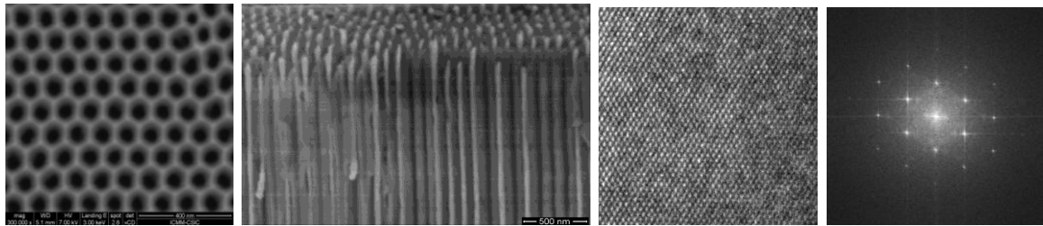
SEM images of anodic template (far left) and Co nanowire array (middle left). HRTEM image of single crystal hcp Co nanowire and its FFT
