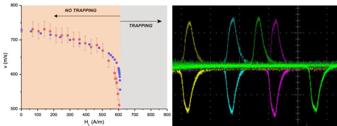
Left.- Domain wall velocity in a FeSiB microwire is tuned in with a local field, H_L , antiparallel to the homogeneous drive field originating the wall motion. For a given local field, 610 A/m, it gets trapped. Experimental and calculated data of DWSt speed are included ( M. Vazquez et al. Phys. Rev. Letters, 108 (3), art. no. 037201 (2012) ) Right.- Sequences of induced signals at the pickup coils numbered (yellow, blue, pink, green), under rightward (bottom peaks) and leftward (upper peaks) applied field of amplitude 392 A/m. Note the presence of two domain walls moving in opposite directions ( A. Jimenez et al. European Phys. Journal B, 86 (3), art. no. 113 (2013) )
