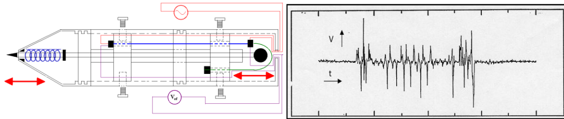
Magnetoelastic Signature device (pen) for signature identification and authentication and magnetoelastic signature (right) using GMI effect glass-coated microwire as sensing element (Patented).
