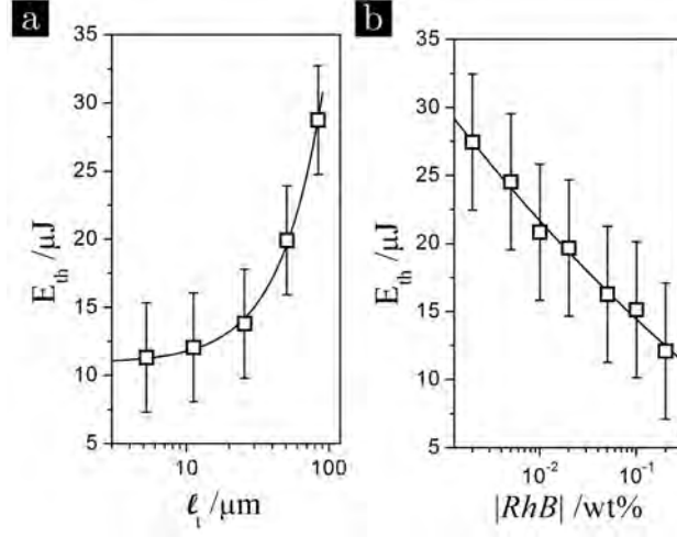
Figure 5.13: a) Dependence of the energy threshold of a set of samples on l_t , for a fixed RhB amount (0.2 wt%). b) Dependence of the energy threshold of a set of samples on RhB concentration, for a fixed titania quantity of 5 wt%.
