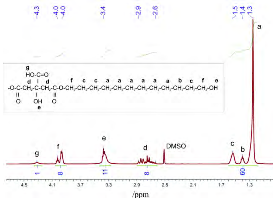
Figure 4.2: Representative ^1\text{H} -NMR spectrum of the PDDC-HD prepolymer. The inset identifies the labels adopted for the chemical shifts characteristic of the different types of groups.
