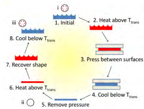
Figure 4.13: Scheme of the protocol followed for studying the hypothesis of erasing the surface nanotopography and testing self-healing features of the imprinted gratings.
