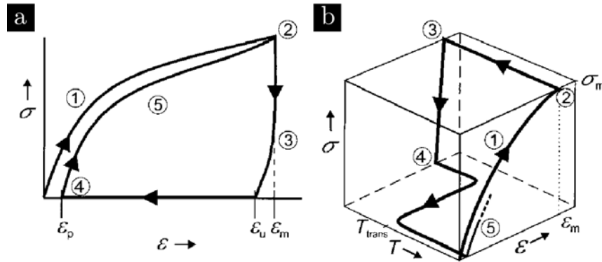
Figure 1.8: Scheme illustrating the two more typical protocols of thermomechanical programming: a) two-dimensional measurement and b) three-dimensional programming. Adapted from [47].
