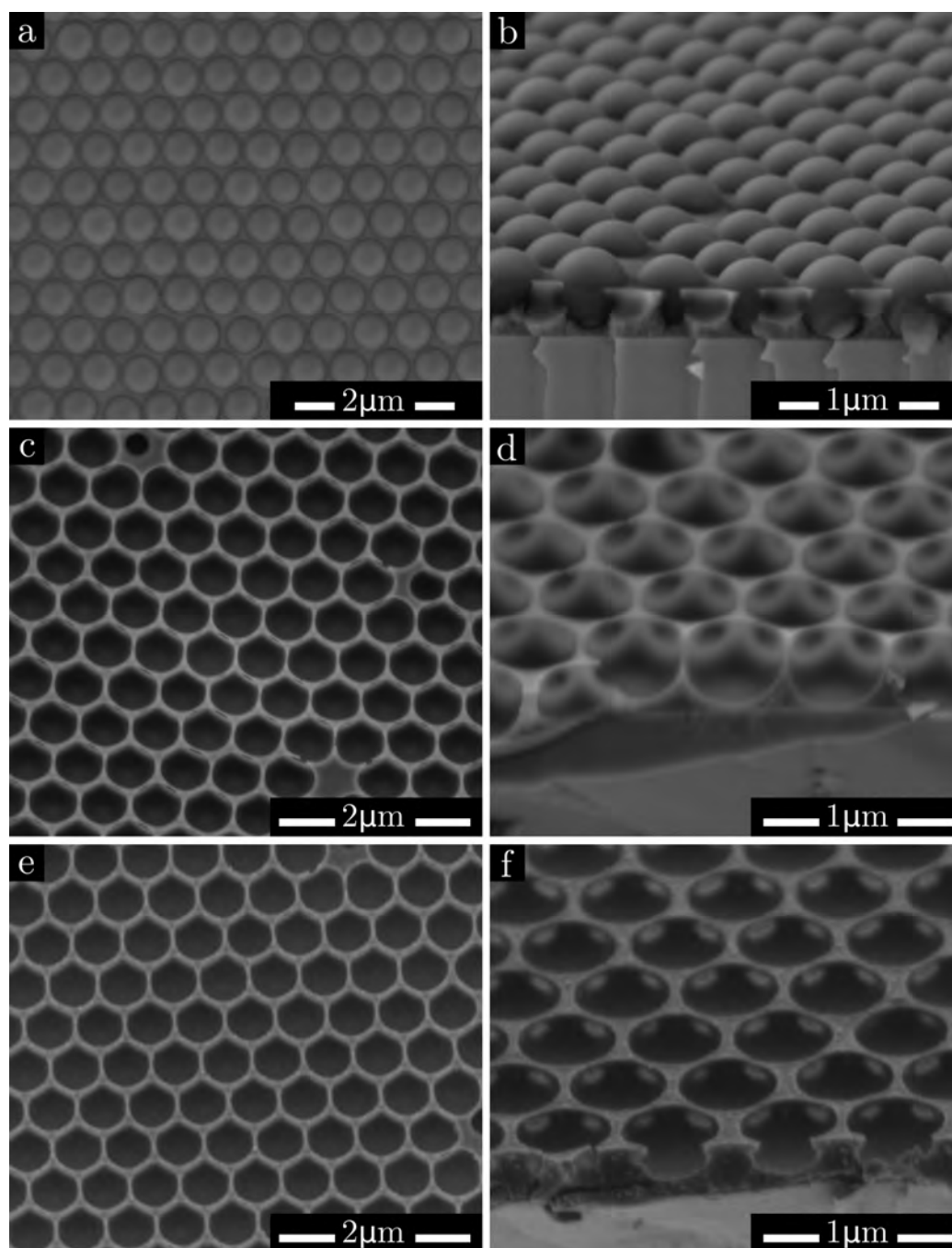
Figure 2.11: Representative SEM images of a crystal produced with spheres of diameter 520 nm and [TEOS] = 4.0 vol%. a) Surface view of the composite, b) tilted angle observation. c) and d) Respective images for the same sample after calcination. e) and f) Respective images after magnesiothermic reduction.
