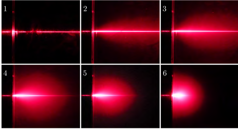
Figure 1.5: A laser beam crossing an homogeneous medium (water) presents ballistic transport. As more and more drops of milk are added to the initial homogenous medium, a colloid is produced and the transport of light changes to diffusive. At a high enough concentration of colloid, the ballistic transport is not observed anymore.
