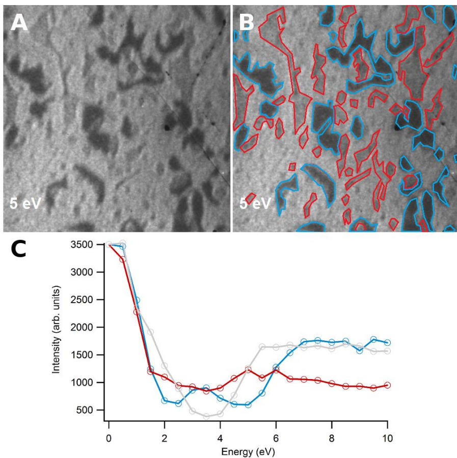
Figure 3 16: a & b. LEEM image of a sample annealed at 1525K where three different contrasts are visible when using 5eV electrons for imaging. The right side presents the same image where the different contrasts have been highlighted for ease the visualization. c. Reflectivity curves for the colored regions in the images showing a correlation between the number of minima and the number of stacked graphene layers. 2 \times 2 \mu\text{m}^2 .
