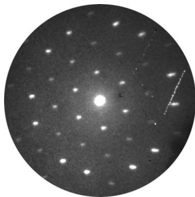
Figure A 6: \mu LEED pattern of the (3x3) taken at electron energy of 80eV .The (1x1) dots are the faint and more external ones.
