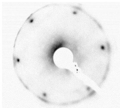
Figure 2 3: Typical G/Pt(111) LEED pattern with an energy of the incident electrons of 130 eV. Dots correspond to Pt(111) (1x1) pattern and the ring-shaped structure results from diffraction of graphene domains with different orientations.
