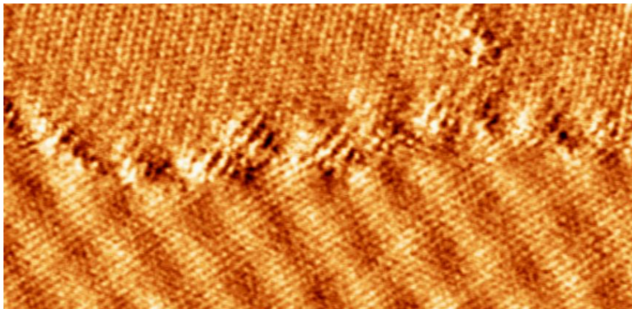
Figure 2 27: Pseudo periodic G-G edge, the grain boundary follows the periodicity of the lower moiré. 18.4 \times 9 \text{ nm}^2 , 2nA, 10mV.
