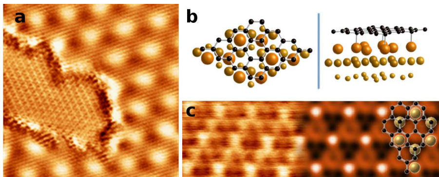
Figure 2 11: a. 12.4 \times 12.4 \text{ nm}^2 STM image showing an island of atomically resolved (\sqrt{3} \times \sqrt{3})R30^\circ or \alpha G/Pt(111) inside a bigger domain of \mu G/Pt(111) Moiré. b. Top view (left) and side view (right) of the structural model derived from DFT calculations for the (\sqrt{3} \times \sqrt{3})R30^\circ reconstruction. Smaller sizes on the orange spheres represent deeper atoms. c. STM images ( V=0.1 \text{ V} ) for the (\sqrt{3} \times \sqrt{3})R30^\circ experimental (left) and DFT best fit simulation (right). A schematic atomic model of where the Pt vacancy network is placed has been overlaid.
