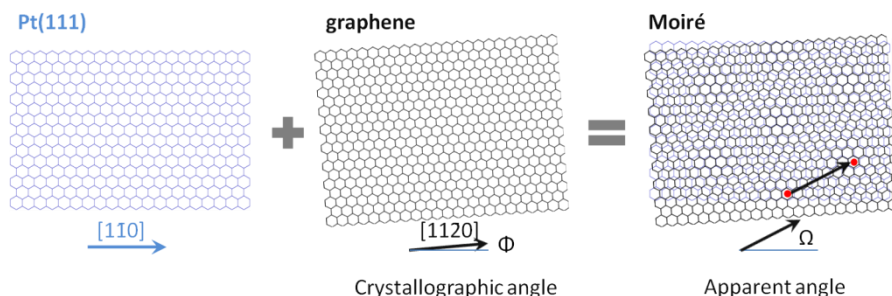
Figure 2 4: Schematic explanation of a hexagonal Moiré. The blue honeycomb lattice represents Pt(111) ( a_{Pt}=2.77 \text{ \AA} ) with one of its main crystallographic directions aligned with the horizontal. The black honeycomb lattice represents graphene ( a_G=2.46 \text{ \AA} ) rotated \Phi (crystallographic angle) respect the Pt directions. When both lattices are overlaid the resulting diagram presents a superperiodicity (Moiré pattern) due to the coincidences (two of them are marked as red dots).
