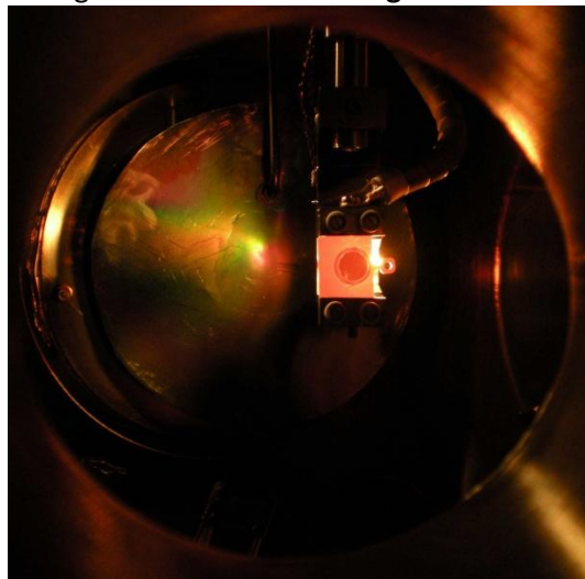
Figure 1 20: Picture of the annealing of the Pt(111) sample. The red-glowing platelet is the sample holder irradiating visible light. The darker orange circle inside the glowing square is the Pt(111) sample at an approximated temperature of 1100K.
