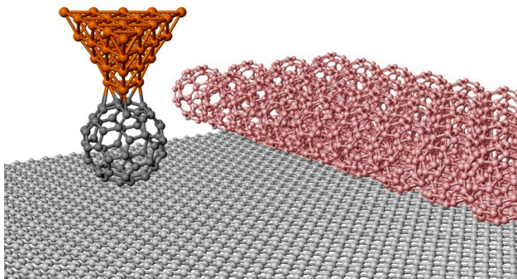
Figure 3 34: Schematically representation of the best agreement model according to the experimental observations. The C_{60} molecules form a 4x4 ordered close-packed superstructure on top of SLG. A C_{60} molecule is attached to the scanning tip.
