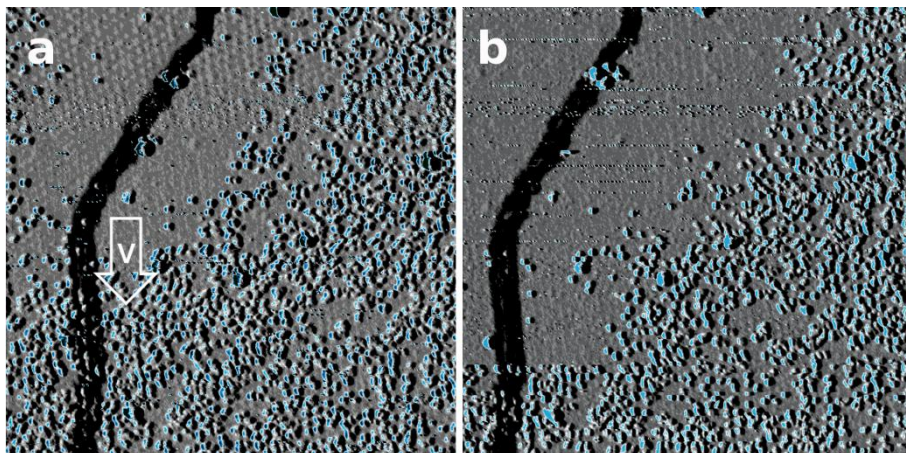
Figure 3 21: Consecutive STM images of a region of H/G/SiC. a. The white arrow marked with a V indicates the place where a voltage pulse of 4 V was performed, V=2.2\text{V} , I=1\text{nA} , 80\times 80\text{nm}^2 . b. In this image we observe that the voltage pulse has generated a region clean of atomic adsorbates on the surface V=2.2\text{V} , I=1\text{nA} , 80\times 80\text{nm}^2 .
