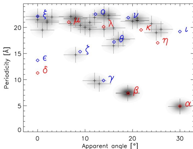
Figure 2 10: Periodicity vs. apparent angle for measured STM images of graphene islands (crosses) together with the predicted Moirés (rhomboidal ticks and Greek letters). The vertical and horizontal grey lines are the error bars of the experimental determination of periodicities and Moiré angles in STM images, respectively. 2D Gaussian shapes with intensity proportional to the experimental count of finding a Moiré with a given angle and periodicity are superimposed. The interpretation of the figure can be seen as a histogram where the colour intensity of a point is proportional to the occurrence of a structure.
