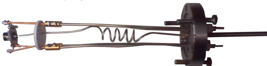
Figure 1 19: Picture of our home-made H-cracker. The hydrogen is introduced through the serpentine and the rest of Cu contacts serve to pass the high voltage as well as for passing current through the filament.
