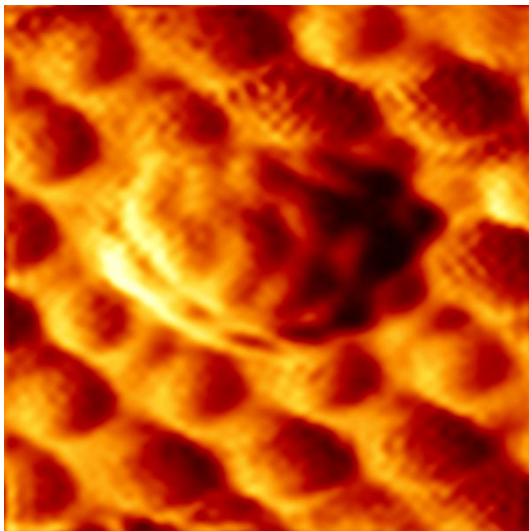
Figure A 12: High resolution STM image of a single fullerene adsorbed onto (3x3)/SiC(0001) surface. V=-3V , I=0.1nA , 4 \times 4 nm^2 .
