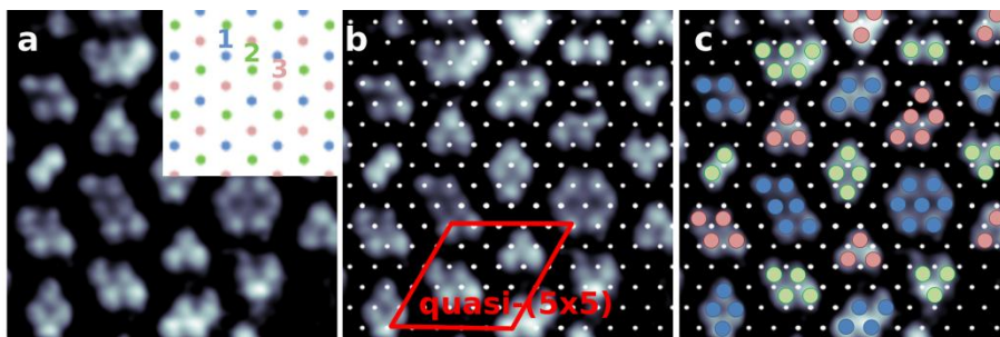
Figure 3 7: Explanation model of the quasi-(5x5) superstructure .a. The STM image as recorder (filtered for ease the visualization). Inset: scheme of the three nonequivalent ( \sqrt{3}\times\sqrt{3} ) R30^\circ lattices, blue (1, white in the b and c images), green (2), and red (3). b. One of the three sublattices is represented with white dots, the other two sublattices correspond to the middle of the triangles, on a when the triangles are looking upwards, and the other when the triangle are looking downwards. Every sublattice is represented with a different color: blue, green, and red. c. The tree lattices are represented.
