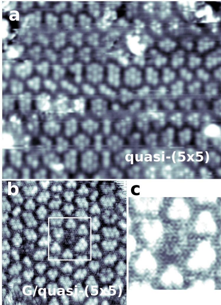
Figure 3 8: STM images of the quasi-(5x5)/SiC(0001) reconstruction and the G/quasi-(5x5)/SiC(0001). a. 20 \times 16 \text{ nm}^2 , -3400 \text{ mV} . b. In this image the reconstruction is covered by a graphene overlayer, the white square marks the region highlighted in c, 14 \times 14 \text{ nm}^2 , -400 \text{ mV} . c. Detail of the b image corresponding to the white square in b, where the graphene lattice is visualized as a small corrugation, 5 \times 5 \text{ nm}^2 , -400 \text{ mV} .
