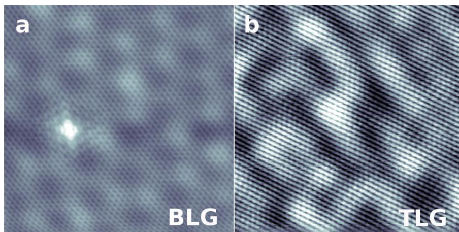
Figure 3 19: STM images of multilayer graphene on SiC(0001). a. Bilayer graphene where subsurface buffer layer structure is not visible but the Moiré-like long range pseudoperiodicity is still conserved. An atomic scale defect- probably involving two pentagons- is spotted in the center-left of the image. 10 \times 10 \text{ nm}^2 , -1100 \text{ mV} . b. A region with small corrugation of graphene is clearly visible and probably consisting of 3 -or more- layers of stacked graphene, 10 \times 10 \text{ nm}^2 , -100 \text{ mV} .
