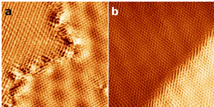
Figure 2 28: Examples of 1D defective . G-G edge vs. graphene running through a Pt step. a . 10 \times 10 \text{ nm}^2 1.9nA, 10mV. b . 7.5 \times 7.5 \text{ nm}^2 , 8nA, 2mV.
