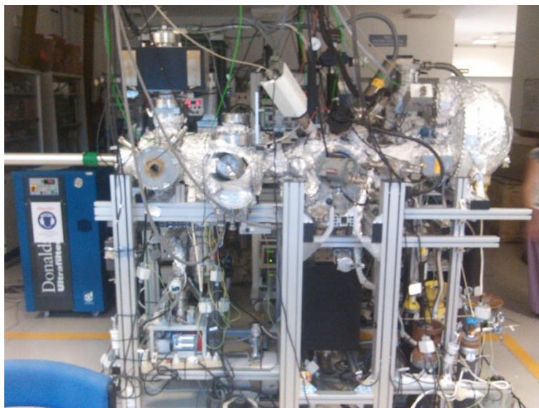
Figure 1 24: Picture of the combined microscopy and photoemission chamber held by the Centro de Astrobiologia.
