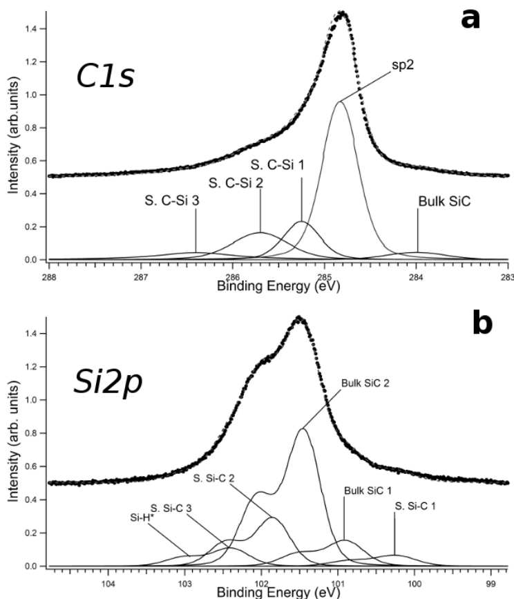
Figure 3 14: a. XPS spectrum of the C1s peak of G/SiC sample annealed at 1400K recorded at a photon energy of 400eV. b. XPS Spectrum of the Si2p peak of G/SiC sample annealed at 1400K recorded with a photon energy of 150eV.
