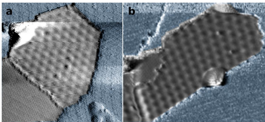
Figure 2 18: STM images showing graphene edges running parallel to their Moiré apparent angles. Nanobubble or graphene folds can be seen in the islands. a. 30\times 30\text{nm}^2 , 2nA, -100mV. b. 30\times 25\text{nm}^2 , 1nA, 50mV.
