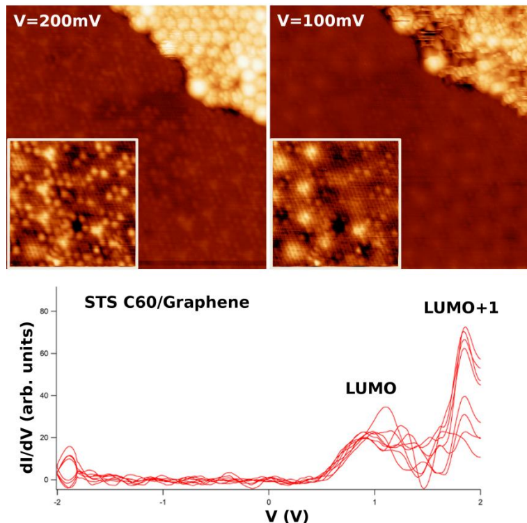
Figure 1 7: upper part, 20 \times 20 \text{ nm}^2 STM images at two different bias of C_{60} molecules (upper right corner) and graphene showing differences with voltage. At 100mV the fullerenes do not have significant DOS and thus electrons from the tip cannot tunnel to them, while at 200 mV the fullerenes have more states but graphene instead does not and looks transparent (detail presented in the lower insets). Lower part, dI/dV spectrum of C_{60} molecules on SiC. The molecular orbitals in the unoccupied energy region are revealed at around 1V (LUMO) and 1.7V (LUMO+1).
