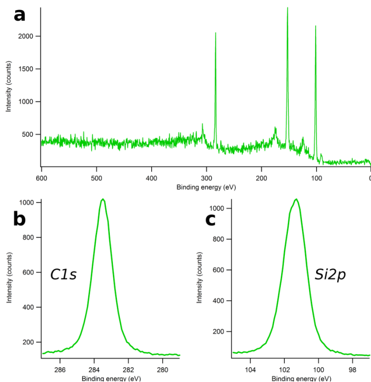
Figure A 8: XPS spectrum of the ( \sqrt{3}\times\sqrt{3} )R30° surface using an Al K \alpha anode (1486.6 eV) as X-ray source and hence the rather low quality . a. Overview for comparing the relative intensity of the C1s and Si2p and Si2s peaks. b. detail of the C1s peak, only one component appears at an energy corresponding to carbide. c. Si2p peak, the second component occurring in the (3x3) reconstruction is absent in here.
