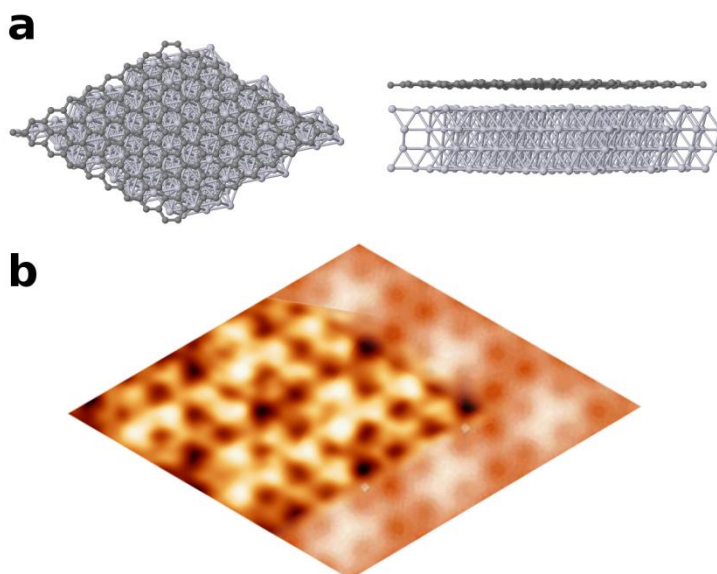
Figure 2 13: Extended structure of the (v7 \times v7)R19^\circ Moiré. a. Ball and stick model of four contiguous unit cells. b. Simulated STM image at 0.1V bias for the extended structure where the (3 \times 3)_G periodicity is clearly resolved together with an experimental image taken at 0.1V.
