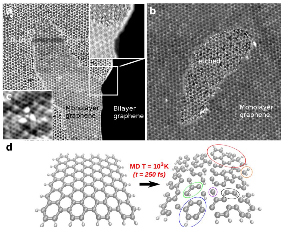
Figure A 15: STM images after H dosing at 1100 K of G/SiC and computer simulation of the proposed etching process. a. 100 \times 100\text{ nm}^2 , -1100\text{ mV} . Wide view of a region where the graphene has been reduced to a stripe with rounded edges on the center of the image. On the right part of the image a region of bilayer graphene seems unaltered. The upper inset shows a high-resolution image of a kink where SLG, BLG and the modified etched substrate coexist. b. STM image of a hole in the middle of a graphene terrace. These holes are observed after H treatment at high temperatures and they evidence etching through edges and defects. 70 \times 70\text{ nm}^2 , -1.1\text{ V} . c. Atomically resolved STM image of a subsurface trimer 2.5 \times 2.5\text{ nm}^2 , -400\text{ mV} . d. Initial and final frames of the graphene surface extracted from a movie of DFT molecular dynamics calculations of the G/H/SiC system. The distance between graphene layers expand from 7% at room temperature to about 62% at 1000K, and finally, after 250 fs (MD time), the topmost layer disrupt in the form of small carbonaceous species. In this case benzene rings (blue oval), acetylene molecule (black oval), methylene radical (orange oval), or PAHs (red oval) can be identified.
