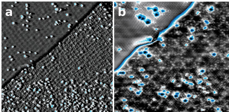
Figure 3 20: STM images of the H/G/SiC system in a region where bilayer(top-left) and single layer(bottom-right) graphene coexist. H binds to both reconstructions with a similar sticking factor. a. V=-0.6V , I=1nA , 40 \times 40 nm^2 . b. V=-0.2V , I=1nA , 20 \times 18 nm^2 . A double color scale is used for this image where both terraces (upper and lower) correspond to different color scales. This image treatment was performed to ease the visualization of the atomic resolution in both surfaces.
