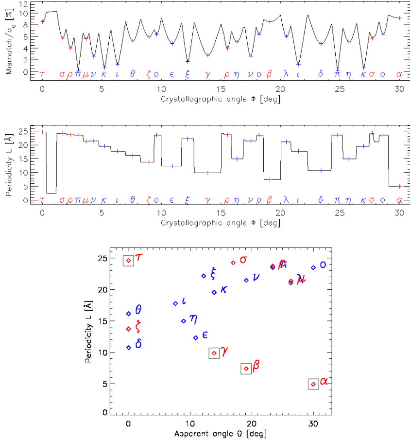
Figure A 2: Figure caption. Stability plots for G/Ir(111). The structures marked with solid squares are found experimentally in ref. 4
