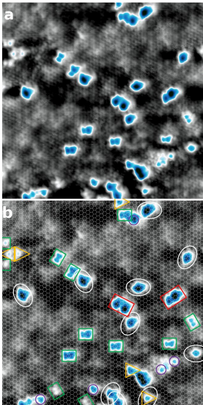
Figure 3 23: High resolution STM images of hydrogen adsorbates on SLG forming small clusters. a. V=-0.3\text{V} , I=1\text{nA} , 12\times 12\text{nm}^2 . b. Image where the atomic graphene grid has been superimposed and the clusters have been classified by a color code.
