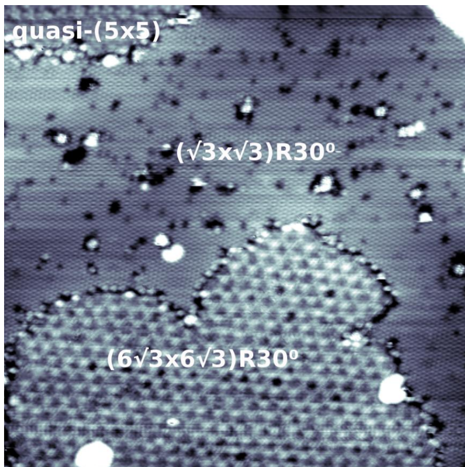
Figure A 10: STM image where different reconstructions of the SiC(0001) coexist. In the upper-left corner an island of quasi-(5x5) reconstruction is found. In the middle region the (\sqrt{3} \times \sqrt{3})R30^\circ reconstruction dominates, although lots of defects are spotted. On the lower part of the image an area with the (6\sqrt{3} \times 6\sqrt{3})R30^\circ reconstruction is found. 50 \times 50 \text{ nm}^2 , 2500mV.
