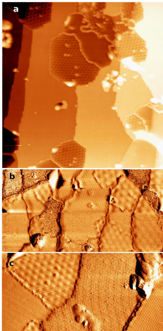
Figure 2 5: STM images of the G/Pt(111) systems formed using C_{60} as precursors at 1150K. a. 100x100 nm 2 topographic image, V=400\text{mV} , I=0.2\text{nA} . The flat regions correspond to clean Pt(111) surface whilst the hexagonal corrugated regions correspond to the Moiré superstructures with different apparent angles. b. 50x25 nm 2 current signal error image, V=300\text{mV} , I=0.1\text{nA} . The smooth regions correspond to graphene with different rotational domains, whereas the clean Pt(111) regions look spiky in these imaging mode. c. 50x25 nm 2 signal error image, V=-100\text{mV} , I=2\text{ nA} .
