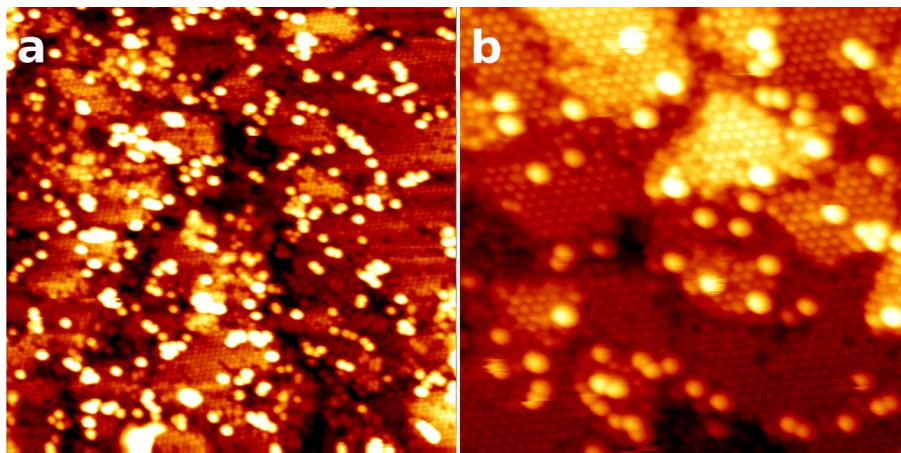
Figure A 11: STM images showing C_{60} molecules adsorbed onto the Si-rich (3x3)/SiC surface. a. V=-3V , I=0.1nA , 75 \times 75 nm^2 . b. V=-3V , I=0.2nA , 35 \times 35 nm^2 .
