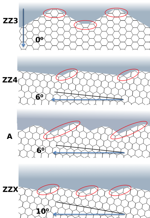
Figure 2 17: Schematic model of the preferred graphene termination of border-like at the G-metal interface. The blue side corresponds to the Pt region, with crystallographic direction, indicated by a blue arrow, along the horizontal (except for ZZ3, where it is along the vertical). The graphene tends to adopt zigzag configurations by minimizing the number of armchair unit cells for a given crystallographic angle with respect to the Pt surface. Armchair configurations are marked with red ovals.
