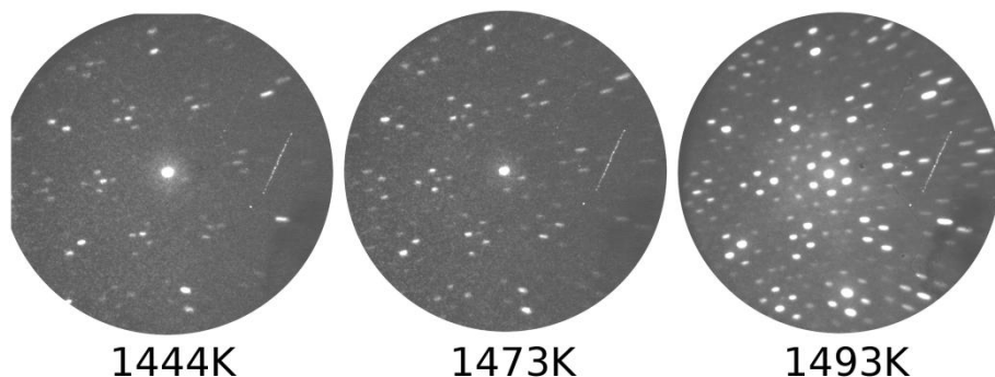
Figure 3 15: \mu -LEED pattern of the surface annealed at slightly different temperatures, showing great variation in a small temperature range.
