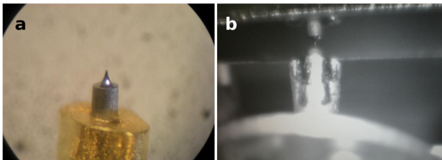
Figure 1 6: STM tips under optical microscope. a. A commercial tip mounted onto a gold-coated tip-holder. b. A tip during scanning into the microscope. The reflecting surface corresponds to a SiC sample.
