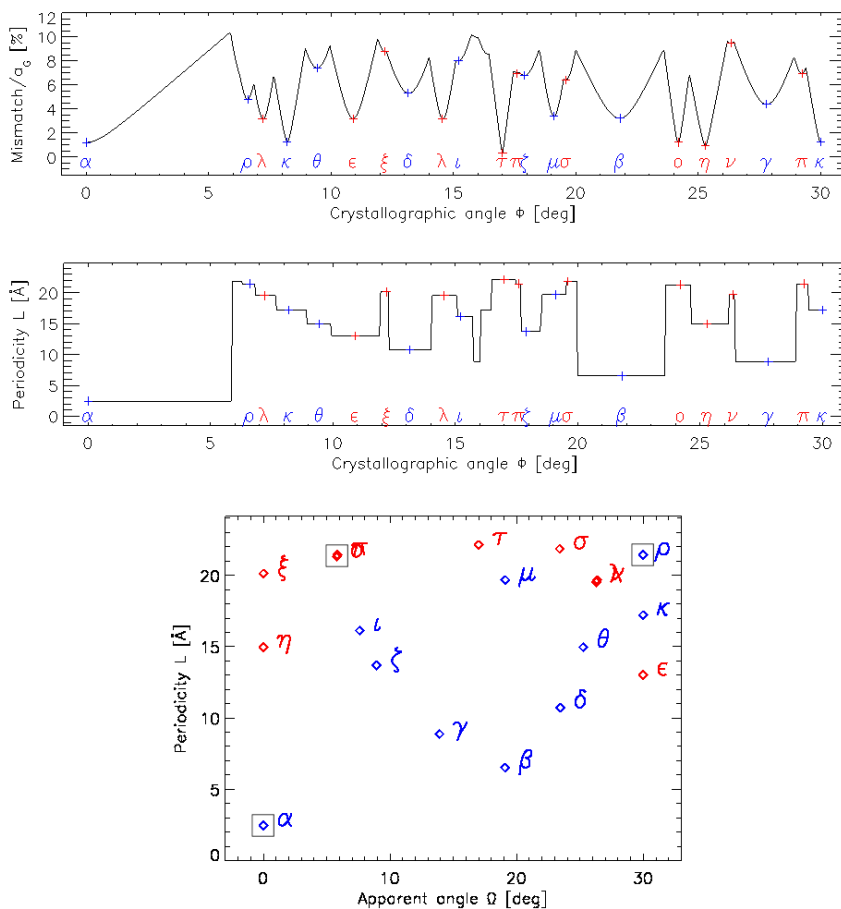
Figure A 3: Stability plots for G/Ni(111). The structures marked with solid squares are found experimentally in refs. 5 6 .
