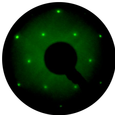
Figure A 9: LEED pattern of the (\sqrt{3} \times \sqrt{3})R30^\circ/\text{SiC}(0001) surface.
