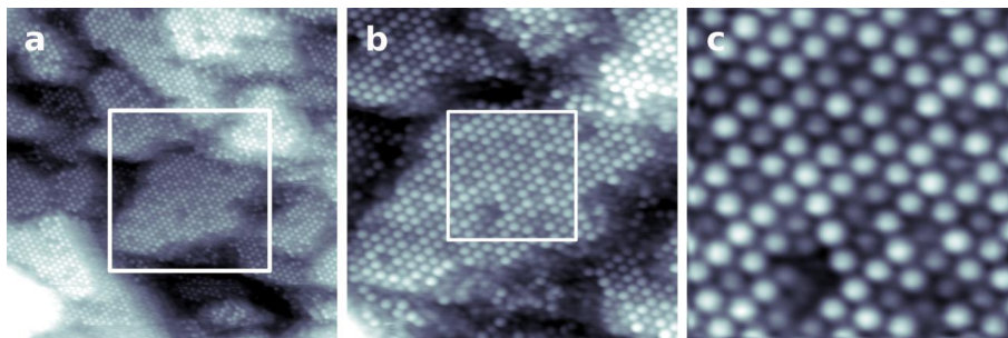
Figure A 4: STM images showing the terrace morphology and atomically resolved images of the (3\times3)/\text{SiC}(0001) reconstruction. The white square in a (b) corresponds to the region shown in b (c). a. 50\times50\text{ nm}^2 , 0.2\text{ nA} , -3000\text{ mV} . b. 25\times25\text{ nm}^2 , 0.2\text{ nA} , -3000\text{ mV} . c. 10\times10\text{ nm}^2 , 0.2\text{ nA} , -3000\text{ mV} .
