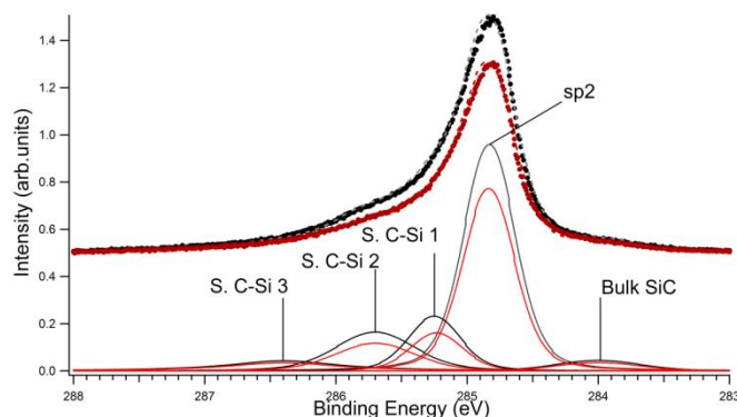
Figure A 16: Synchrotron-based XPS spectra of C1s before (black curve) and after (red curve) H treatment (550L) at 1200K. Beneath the experimental data we show their decomposition into separate components. A decrease in the C peak of about 28% in the surface-related components indicates that those C-species have been etched away through H processing. The component appearing at 284.8 eV can be assigned to the graphene sp^2 configuration. The components located at lower binding energies (about 284.0 eV) are attributed to bulk carbides and the components at the left-hand side of the spectra to the buffer layer (between graphene and SiC). Photon energy: 400eV.
