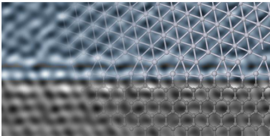
Figure 2 21: Ball and stick model of the DFT relaxed structure compared with the false colored STM image. The atomic positions of the calculations reproduce with great accuracy the protrusions in the STM images .
