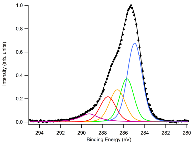
Figure 1 15: XPS deconvolution of graphene oxide. The blue component, centered at 284.8eV corresponds to C in sp^2 configuration; the other components are assigned to different carbon oxidized species. Spectrum acquired under illumination with an Al_{K\alpha} X-ray source (1486.6 eV).
