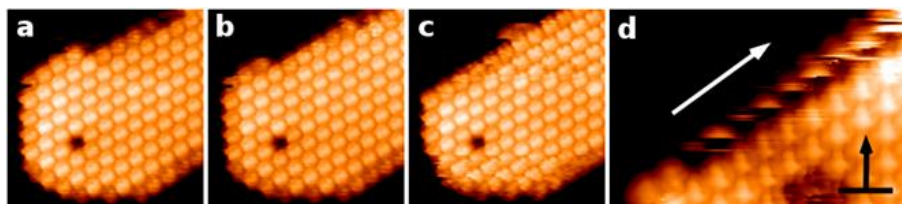
Figure 3 37: a-c. 12 \times 12 \text{ nm}^2 STM topography sequence showing transport of C_{60} molecules one-by-one. d. Movement of one C_{60} along the island boundary (white arrow) caught in one 11 \times 7 \text{ nm}^2 image scanned from the bottom to the top (black arrow). All data taken at 600mV bias voltage and 100pA tunnelling current.
