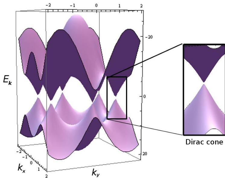
Figure 0 2: Calculated energy band dispersion for the graphene electronic structure. (Right) Closer look to the energy band near the k point in the reciprocal space known as Dirac point, and the so-called Dirac cones.
