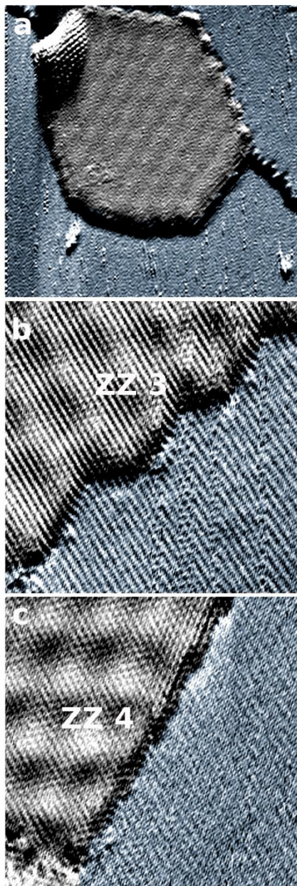
Figure 2 16: a. STM image showing a graphene island, a nanobubble can be seen in the upper part of the flake. 34 \times 34 \text{ nm}^2 , 1.9 \text{ nA} , 100 \text{ mV} . b. Detail of a crystalline edge with a graphene zig-zag termination, 10 \times 10 \text{ nm}^2 , 3.94 \text{ nA} , 10 \text{ mV} . c. Detail of a crystalline edge with a graphene zig-zag termination, 10 \times 10 \text{ nm}^2 , 3.94 \text{ nA} , 10 \text{ mV} .
