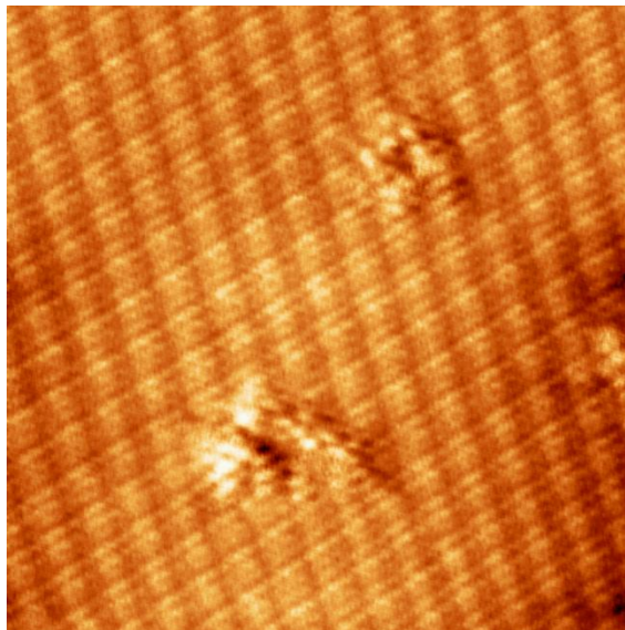
Figure 2 25: STM images showing two 0D defects on graphene on Pt(111). These structures are present in small patches of graphene with high strains. 12x12nm, 100mV, 1nA.
