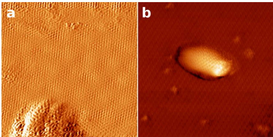
Figure 2 29: Examples of 2D defective structures. a. Surface carbide, 10 \times 10 \text{ nm}^2 , 8 \text{ nA} , 2 \text{ mV} . b. Graphene nanobubble, 20 \times 20 \text{ nm}^2 , 0.6 \text{ nA} , 310 \text{ mV} .
