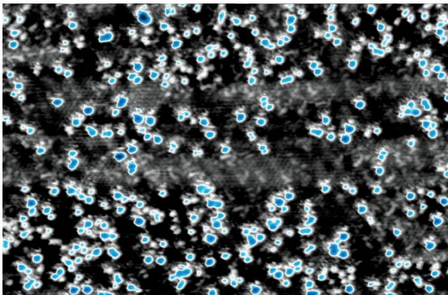
Figure 3 22: STM image of hydrogen adsorbates on SLG where some identifiable structures seems to be repeated. More than 350 clusters are shown occupying 15% of the total area. V=-0.1V , I=1nA , 40 \times 26 nm^2
