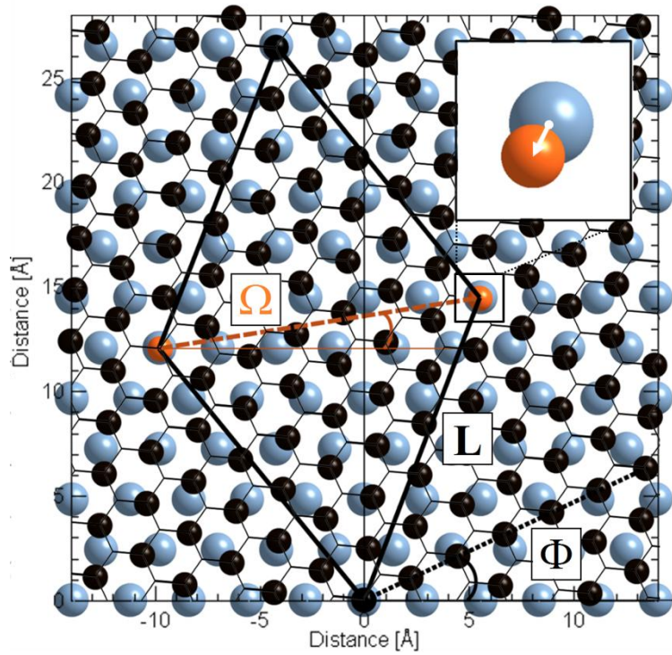
Figure 2 7: Diagram of the model represented for the \zeta\text{G}/\text{Pt}(111) superstructure. Pt atoms are represented by blue spheres whereas one hexagonal sublattice of graphene is represented by black spheres. The angle between the black dotted line and the Pt [1\bar{1}0] surface direction (x axis) represents the crystallographic angle, \Phi , which is equal to 25.1^\circ for this particular case. The orange spheres are the carbon atoms with the lowest mismatch, which define the Moiré unit cell for a given \Phi indicated by the black rhombus. The angle between the orange dashed line and the Pt [1\bar{1}0] direction is the Moiré apparent angle ( \Omega ). The white arrow in the inset represents the mismatch.
