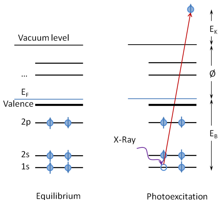
Figure 1 14: Schematic representation of the photoelectric effect. The Sketch shows the working principles of XPS. A photon excites a core-level electron above the vacuum level. The kinetic energy of the outgoing electron is recorded and the binding energy can be calculated.
