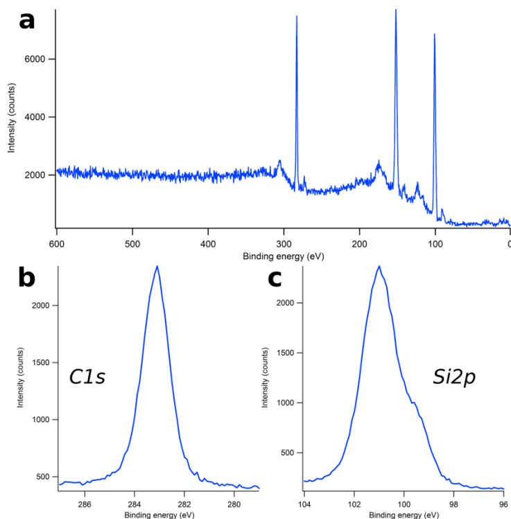
Figure A 5: XPS spectra of the (3x3)/SiC(0001) surface using an Al K \alpha anode (1486.6 eV) as X-ray source. a. Overview for comparing the relative intensity of the C1s and Si2p and Si2s peaks. b. detail of the C1s peak, only one component appears at an energy corresponding to carbide. c. Si2p peak.
