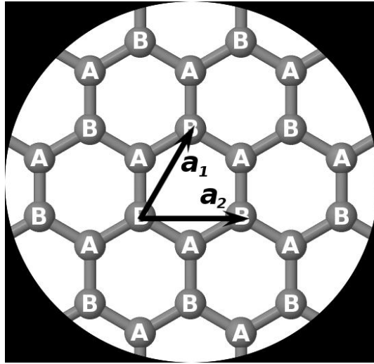
Figure 0 1: Schematic ball-and-stick representation of the honeycomb lattice of graphene. The structure consists of two interpenetrating hexagonal lattices.
