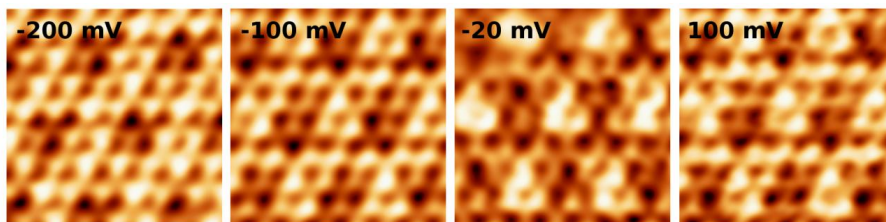
Figure 2 12: Series of 2\times 2\text{nm}^2 STM images of the (\sqrt{7}\times\sqrt{7})R19^\circ Moiré taken at different bias voltages. The bias is written in the upper part of the image. The bias dependence is clearly seen as the bright pockets get narrower near the Fermi level.
