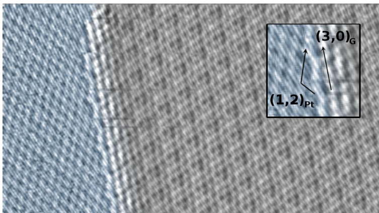
Figure 2 15: High resolution, atomically resolved, STM images of the 8G/Pt(111)-Pt(111) interface. These crystalline edges are energetically favored and might be determinant in the orientation of the possible Moiré superstructures. 12.6 \times 6.8 \text{ nm}^2 , V=40.2\text{mV} , I=5.2 \text{ nA} . The inset shows the chiral vectors of this particular edge.
