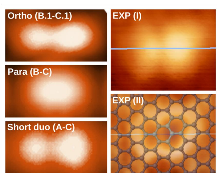
Figure 3 26: Simulated STM images for the different proposed theoretical configurations of the hydrogen dimers together with experimental images (with and without grid) for comparison.
