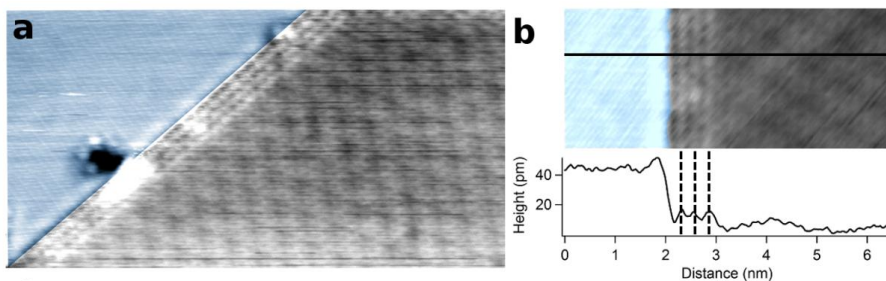
Figure 2 23: a. 13.4 \times 6.9 \text{ nm}^2 Topographic STM image of a border-like edge where an excess of charge is visualized parallel to the interface in the first three rows of graphene V_s = 51 \text{ mV} , I_t = 4 \text{ nA} . b. Detail of such 1D states and height profile.
