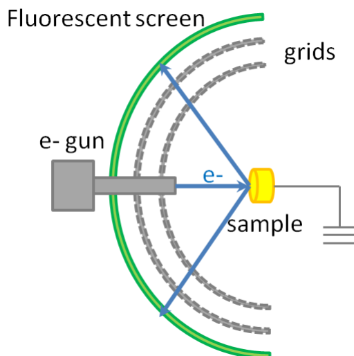
Figure 1 11: Sketch of the basic components of a LEED device. The electrons from the electron gun are accelerated towards the surface and the reflected ones retarded and finally accelerated towards a fluorescent screen showing the interference LEED pattern.
