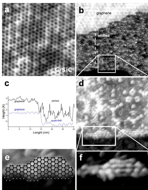
Figure A 14: The surface of stardust SiC is strongly graphitized after formation at temperatures about 1500K and exposure to atomic H produces a strong erosion of this layer. a. 5×5 nm 2 STM image showing a graphene region V=100mV. The small mesh corresponds to the atomic honeycomb atomic lattice of graphene. b. The image shows at the upper side a graphene plane whereas at lower part the surface has strongly roughen. 40×40 nm 2 V=-100mV. c. Profile on STM images recorded before (blue) and
