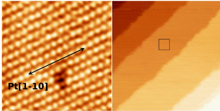
Figure 1 21: STM images of clean Pt(111) surface. a. 5 \times 5 \text{ nm}^2 Atomically resolved high resolution image where every of the protrusions corresponds to a single Pt atom. b. 50 \times 50 \text{ nm}^2 image showing straight atomic steps, the small black square corresponds to the area marked in the a image.
