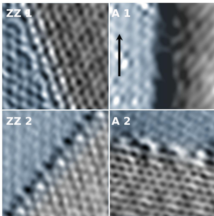
Figure 2 20: Atomically resolved current (signal-error) STM images of: ZZ1) the zigzag edge number 1; I_t = 5.2\text{nA} , V_s = 38\text{mV} ; A 1) the amorphous edge number 1; I_t = 2.4\text{nA} , V_s = 42\text{mV} , the arrow indicates the Pt[ \bar{1}\bar{1}0 ] direction; ZZ 2) the zigzag edge number 2; I_t = 3.8\text{nA} , V_s = 47\text{mV} ; and A 2) the amorphous edge number 2; I_t = 5.2\text{nA} , V_s = 38\text{mV} . Blue/grey regions are identified by the lattice symmetry to be Pt/G respectively. A boundary region of 3-4 atomic rows is also clearly observed with atomic resolution. These images have been drift corrected and FFT filtered.
