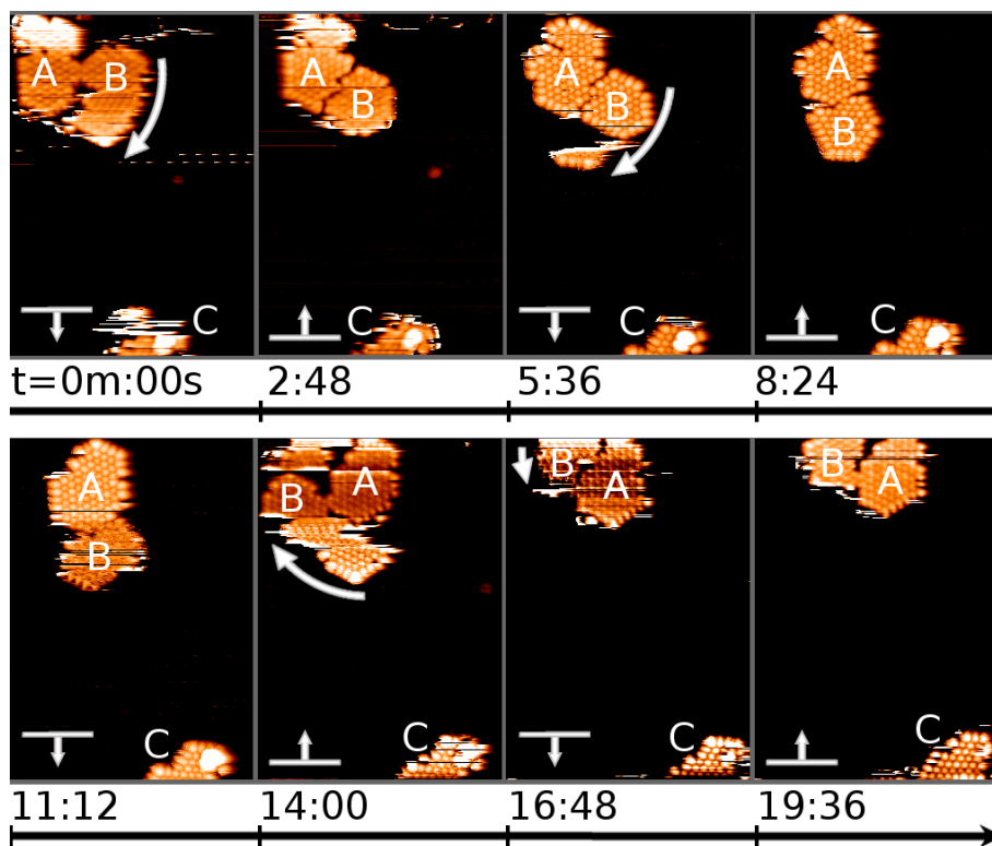
Figure 3 36: Sequence of STM topographic images taken at 1500mV and 100pA on SLG with three islands of C_{60} . Islands A and C are pinned by a step edge and a surface defect respectively. The whole island B is undergoing
