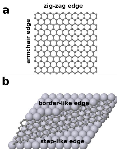
Figure 2 14: Schematic representation of the different graphene edges. a. zig-zag and armchair b. border-like, bounded to the uppermost terrace and step like, lying on top of the bottom terrace.
