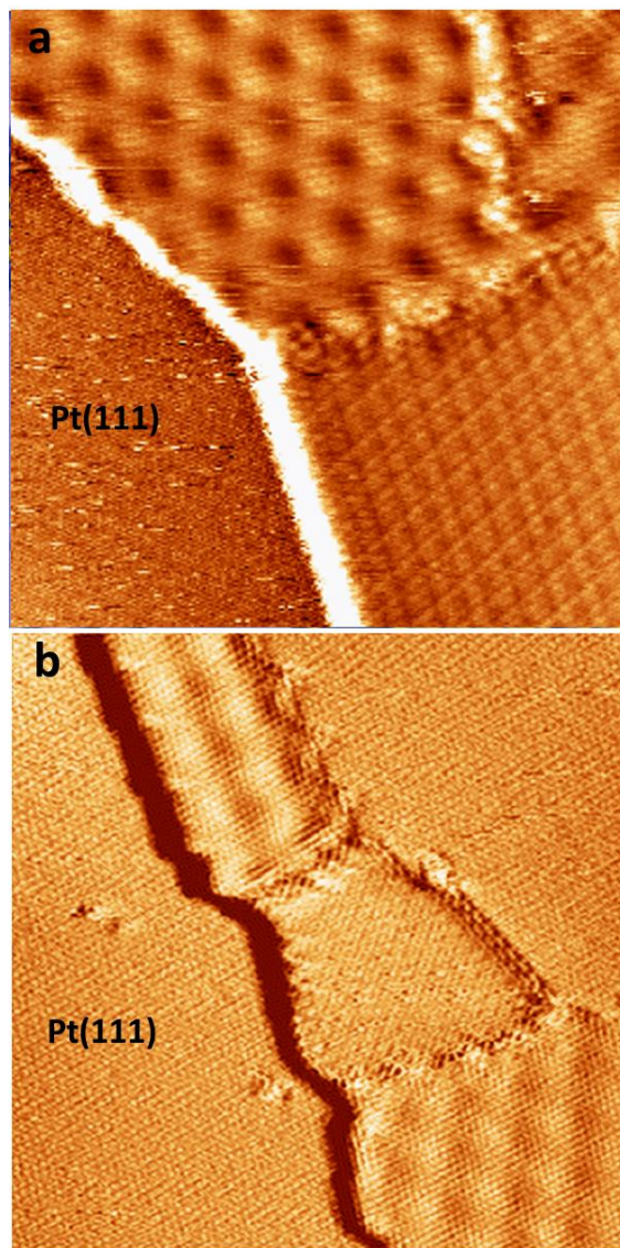
Figure 2 6: Constant current STM images of submonolayer graphene domains on Pt(111). Different graphene superstructures coexist together with clean Pt regions. a. 14 \times 14 \text{ nm}^2 , V=100 \text{ mV} , I=2 \text{ nA} . b. 20 \times 20 \text{ nm}^2 , V=10 \text{ mV} , I=3.9 \text{ nA}
