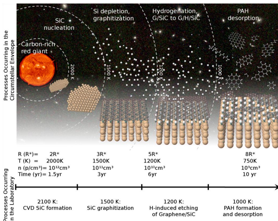
Figure A 13: Qualitative sketch of the proposed model for a novel approach to the formation of interstellar PAHs and related molecules in the envelope of an evolved star. The process can be divided into four different stages. (1) Formation of SiC in the gas phase and condensation into micrometer and nanometer sized grains ( T=2000\text{K} ; 1-5 R^* ). (2) Annealing of the SiC dust grains due to the proximity of the star and the consequent promotion of surface C-rich phases and graphene ( T=2000-1500\text{K} , 1-5 R^* ). (3) Exposure of the surface to atomic hydrogen, promoting graphitization of the C-rich surface and H passivation of the underlying buffer layer ( T=1500-1200\text{K} ; 5-20 R^* ). (4) Etching of the graphene by atomic hydrogen and thermally assisted desorption of PAHs ( T=1200-1000\text{K} , 5-20 R^* ). Temperature values are taken from ref. 38. Lower row: typical temperature in laboratory experiments.
