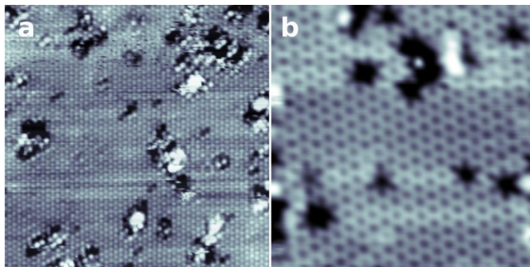
Figure A 7: STM image showing the (\sqrt{3}\times\sqrt{3})R30^\circ reconstruction of the SiC(0001) surface. Several defects are visible in both images, indicating that the surface stoichiometry is lower in [Si] than the nominal value. a. Overview image with “normal” contrast, 25\times 25\text{ nm}^2 , -3500mV. b. Detail image with inversed contrast, probably due to a tip effect, 10\times 10\text{ nm}^2 , -3500mV.
