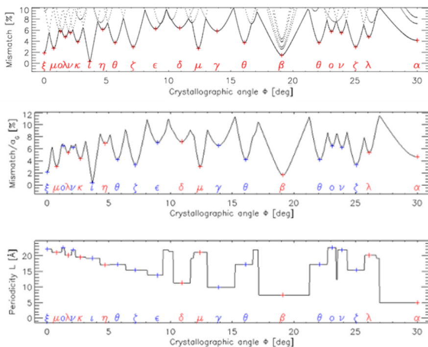
Figure 2 8: (top and middle diagrams) Relative mismatch vs. crystallographic angle ( \Phi ). The solid line indicates the minimum mismatch for the given angle. The dashed lines correspond to coincidence pairs with the lowest mismatch. The blue crosses indicate the stable structures of the model with positive mismatch (tensile strain), while the red ones represent the negative mismatch (compressive strain) phases. These phases are labelled with an associated Greek letter underneath. (bottom) Periodicity, L vs. crystallographic angle \Phi .
