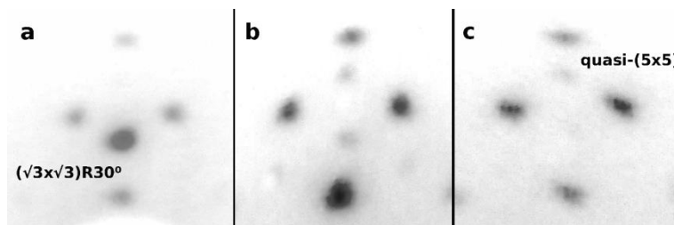
Figure 3 6: Evolution of the inner diamond with temperature (and/or time) as the (\sqrt{3}\times\sqrt{3})R30^\circ spot- the one inside the diamond in the lower half- disappears and the quasi-(5x5) spot – the one inside the diamond in the upper half- appears. In b. we see an intermediate step where both structures coexist in the LEED pattern. The images correspond to different samples and electron energies.
