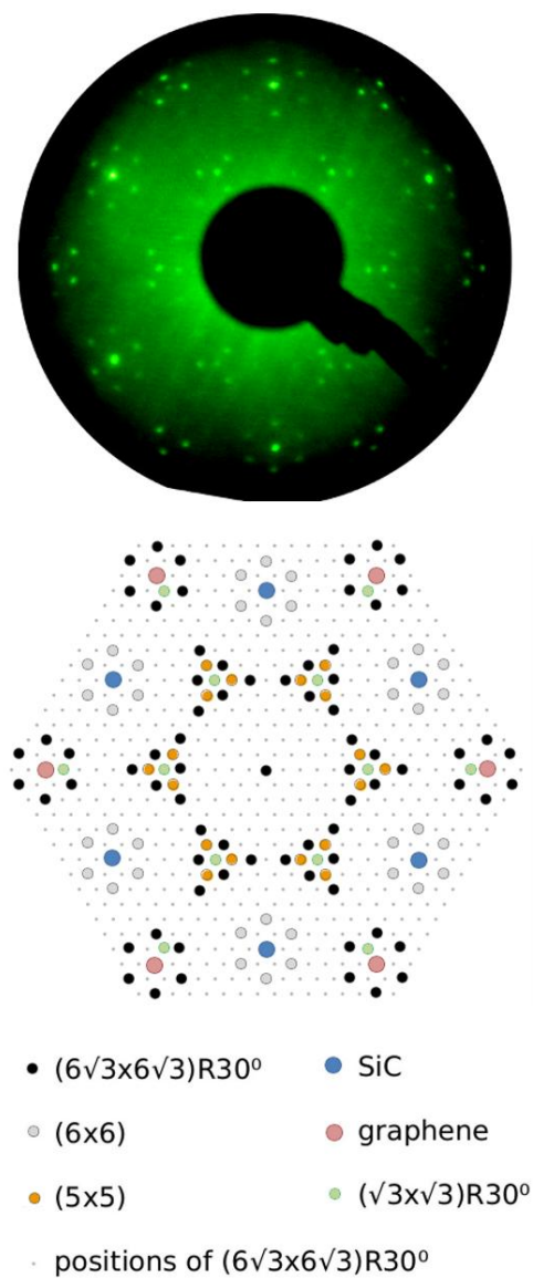
Figure 3 5: LEED pattern of the (6\sqrt{3} \times 6\sqrt{3})R30^\circ structure at 140eV. The theoretical explanation of the pattern is adapted from ref. 20
