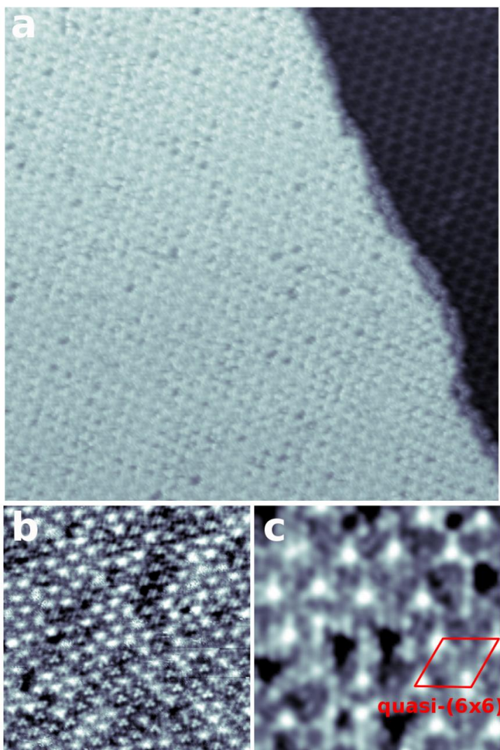
Figure 3 3: STM images of the (6\sqrt{3}\times 6\sqrt{3})R30^\circ reconstruction. a. 50\times 50\text{ nm}^2 , -1200\text{mV} . b. 25\times 25\text{ nm}^2 , -2400\text{mV} . c. 10\times 10\text{ nm}^2 , 1000\text{mV} .
