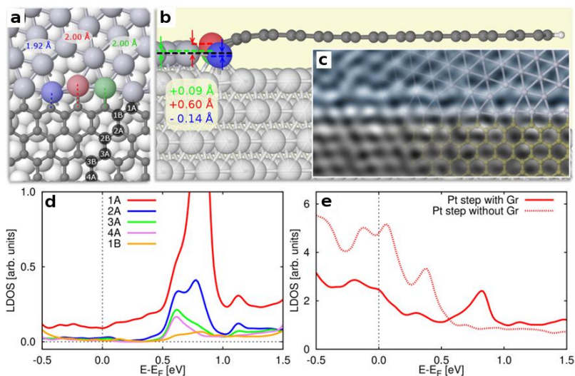
Figure 2 22: a and b . Ball-and-stick model of the atomic configuration of graphene on the Pt(111) step edge calculated with DFT. Bond distance, a , and out of plane displacement, b , of the Pt edge atoms are indicated. c . Overlay of the relaxed structure with the STM image for edge ZZ1. d . Local density of states (LDOS) for the 1 st (red), 2 nd (blue), 3 rd (green) and 4 th (pink) rows of carbon atoms belonging to the same sublattice and for the 1 st (orange) one of the other sublattice. An electronic state at +0.8 eV above E_F is clearly observed only in one sublattice and is mainly localized on the edge row. e . Local density of states (LDOS) for the Pt atoms at the edge of the step that are bonded to the C atoms (solid red) versus the same atoms in a step without a graphene flake attached (dashed red). The same localized electronic state shown in c can be observed in the Pt atoms of our Pt-C system but is absent in the bare Pt step
