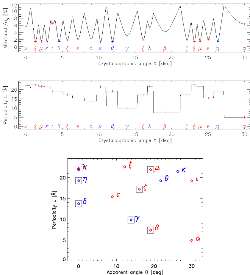
Figure A 1: Figure caption. Stability plots for G/Pd(111). The structures marked with solid squares are found experimentally in 3 .
