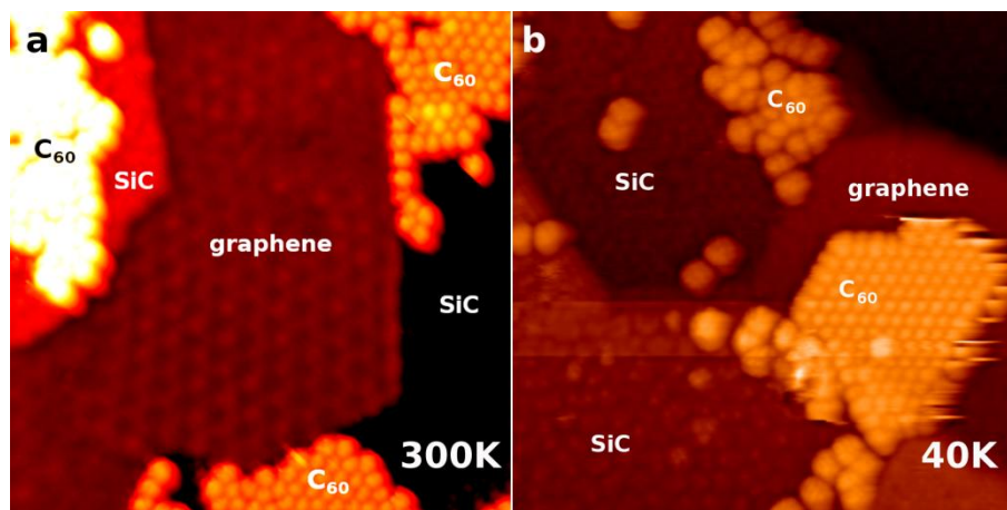
Figure 3 30: STM topography images of C_{60} deposited on a mixture of SiC(0001) phases at a) room temperature, with the C_{60} islands exclusively on the quasi-(6x6) phase and b) at 40 K with C_{60} islands forming also on SLG. The molecules adopt higher order on the SLG compared to the molecules on (6x6). Both images have 30 \times 30 \text{ nm}^2 and were taken at 1.5V bias voltage and 100 pA tunnelling current
