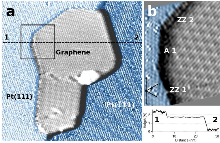
Figure 2 19: a. Topographic STM image ( 31 \times 31 \text{ nm}^2 , sample voltage V_s = 100 \text{ mV} , tunneling current I_t = 3.9 \text{ nA} ) showing a graphene island embedded in a Pt(111) terrace exhibiting three different Moirés. b. Drift corrected current (signal-error) STM image ( 6 \times 8 \text{ nm}^2 , V_s = 42 \text{ mV} , I_t = 2.5 \text{ nA} ) displaying a detailed view of three border-like edges of the squared region in a ). Black arrows indicate the [1\bar{1}0] Pt crystallographic directions. c. Topographic profile corresponding to the dashed line marked in a ).
