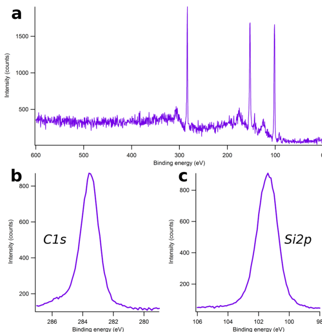
Figure 3 4: XPS spectra of (6V3x6V3)R30° surface using an Al K \alpha anode (1486.6 eV) as X-ray source. a. Overview for comparing the relative intensity of the C1s and Si2p and Si2s peaks. b. detail of the C1s peak, only one component appears at an energy corresponding to carbide, although a small component at higher energies starts to be noticeable. c. Si2p peak.
