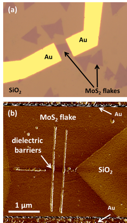
FIG. 3. (a) Optical image of several MoS 2 flakes deposited on a 270 nm thick SiO 2 layer. One of these flakes has been contacted with gold pads by electron beam lithography. (b) AFM phase image of a MoS 2 thin layer FET. The narrowest section of the channel is 200 nm wide. An additional dielectric barrier prevents the current flow outside the channel.
