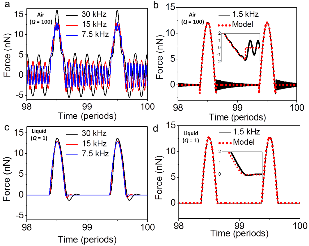
Figure 3. Dependence of the time-varying force reconstructed by using eq 1 on the frequency at which the distance is modulated for air ( Q=100 ) and liquid ( Q=1 ). (a) The sample support is displaced at \omega = 5, 10, 20 ( Q=100 ). (b) The sample support is displaced at \omega=100 ( Q=100 ). The dashed line shows the model force. (c) The sample support is displaced at \omega = 5, 10, 20 ( Q=1 ). (d) The sample support is displaced at \omega=100 ( Q=1 ). The dashed line shows the interaction force (model). The insets show the force in the vicinity of the snap-off region. Simulation parameters, a_0 = 0.2 nm E_{eff} = 1 GPa, H = 0.5 eV, f_0 = 150 kHz, k = 5 N/m, Q = 100 , R = 5 nm, A_m = 15 nm, z_c = 10 nm.
