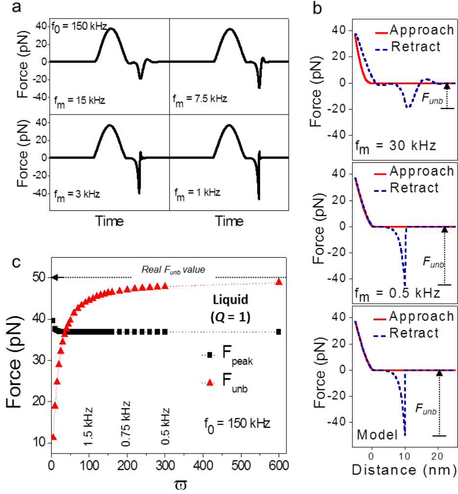
Figure 4. (a) Single-molecule force spectroscopy simulations. Time-varying forces for different distance modulation frequencies in liquid. (b) Force curve reconstructed by using eq 1 for f_m = 30 kHz ( \omega = 5 ) and f_m = 0.5 kHz ( \omega = 300 ) and force curve of the model. (c) Dependence of the unbinding and peak forces on the frequency ratio for f_0 = 150 kHz. Parameters of the interaction force and cantilever dynamics, F_{unb} = 50 pN, \beta = 0.8 \text{ nm}^{-1} , D_0 = 10 nm, a_0 = 0.4 nm, E_{eff} = 1 MPa, k = 0.7 N/m, Q = 1 , R = 5 nm, A_m = 15 nm, z_c = 10 nm.
