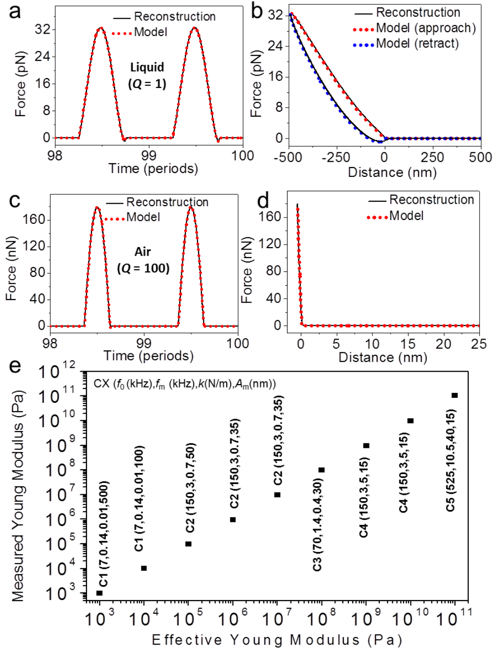
Figure 5. Nanoscale force spectroscopy for soft and stiff materials. Force reconstruction by using eq 1 for a high frequency ratio ( \varpi = 100 ). (a) Time varying force for a cell in liquid ( E_{eff} = 1 kPa). (b) Force versus distance curve deduced from (a). The dashed line shows the model. Simulation parameters, H = 0.0 eV, \eta = 0.1 Pa s, f_0 = 18 kHz, f_m = 0.36 kHz, k = 0.06 N/m, Q = 1 , R = 5 nm, A_m = 500 nm, z_c = 10 nm. (c) Time-varying force for a very stiff sample ( E_{eff} = 100 GPa). (d) Force versus distance curve deduced from (c) The dashed line shows the real (model) force. Simulation parameters, H = 0.3 eV, a_0 = 0.2 nm, f_0 = 525 kHz, f_m = 10.5 kHz, k = 40 N/m, Q = 100 , R = 5 nm, A_m = 15 nm, z_c =
