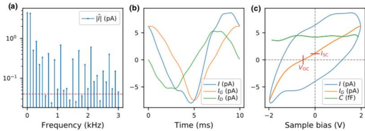
Figure 2: a) Discrete frequency spectrum of the tip-sample current measured in response to a pure cosine voltage waveform. Many harmonics at integer multiples of the excitation frequency are recorded. Only amplitude is shown but a coherent measurement of the phase is made at each frequency. b) Inverse Fourier transform gives the total current I and its two quadrature components corresponding to the galvanic current I_G and the displacement current I_D as a function of time. c) The total current and galvanic current are plotted versus voltage. From the displacement current we also reconstruct the tip-sample capacitance C versus voltage.
