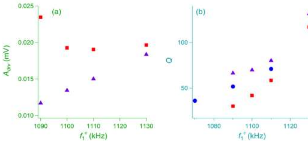
Fig. 1. Median values of amplitude ( A_{drv} ) and Q-factor ( Q ) versus CR frequency: (a) A_{drv} (iso-
