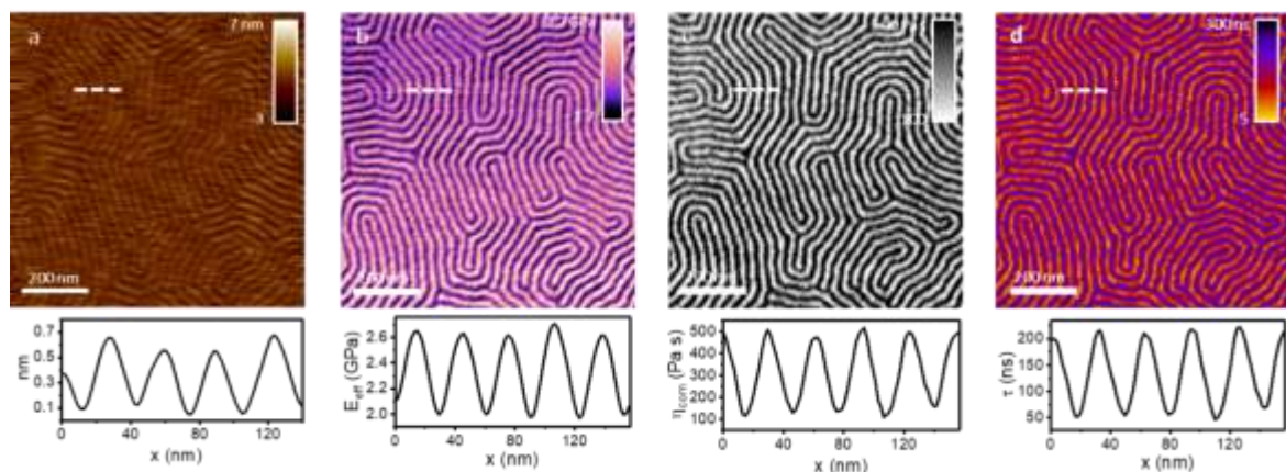
Fig.1 Apparent, deformation and true topography and bimodal nanomechanical maps of a PS-b-PMMA block co-polymer. (a) True topography. (b) Young's modulus. (c) Viscosity coefficient. (d) Retardation time.
