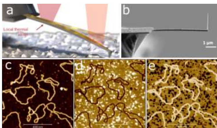
Figure 3: High frequency photothermal off-resonance tapping. a) PORT concept. b) prototype cantilever for MHz PORT. c,d,e) HS-PORT images of plasmid DNA (height, dissipation, adhesion)
