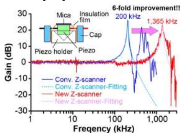
Fig. 1: Comparison of frequency response between the conventional Z-scanner and the new
