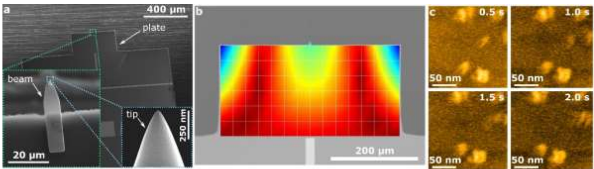
Fig. 1 High-speed scanning probes with high resonance frequency and low stiffness. a SEM image showing the two coupled microstructures. b Vibration mode measured with LDV in air. c Frames of a high-speed AFM video of protein complexes in a buffer solution.
