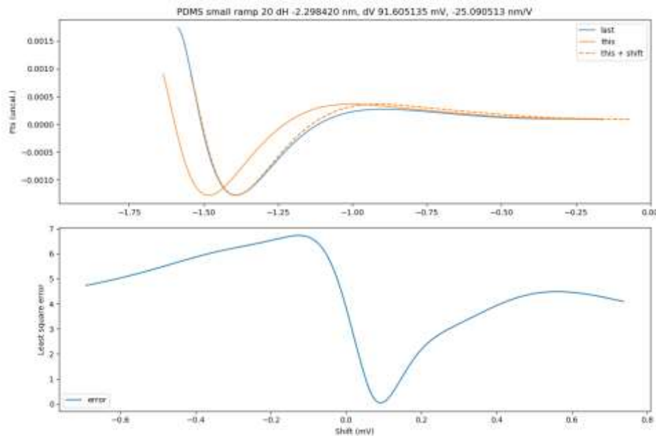
Figure: Top panel, ImAFM force-deflection curves at two different heights (blue and orange). The orange curve has lower peak force and less indentation, but can easily be matched to the blue curve by shifting it along the x-axis (dashed orange). Bottom panel, the shift is found by minimizing or square of the difference between the orange
