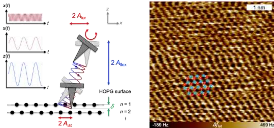
Figure: Schematic illustration of the setup for the nanomechanical characterization of HOPG surfaces via multifrequency atomic force microscopy (left) and lateral frequency shift image, showing atomic resolution of a HOPG surface (right).
