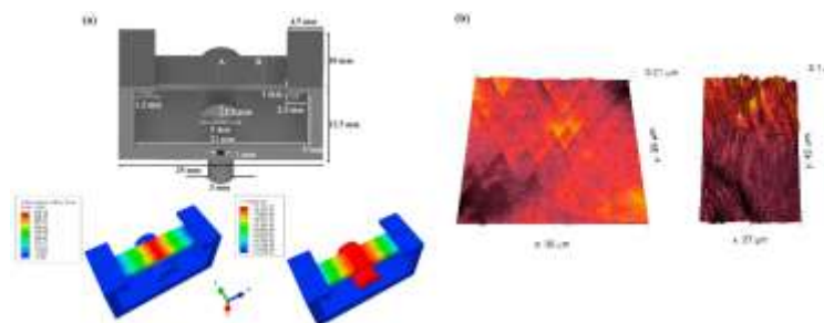
Fig.1. a) Schematic of stage with FE simulation b) HS-AFM map of slip bands after 1000 and 10000 cycles, respectively [4].
