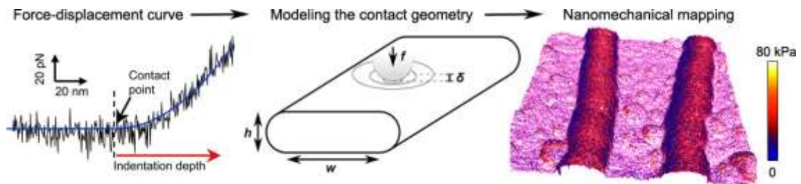
Fig. 1: AFM force mapping and modeling of soft nanotubes gives access to the mechanical properties (tension
