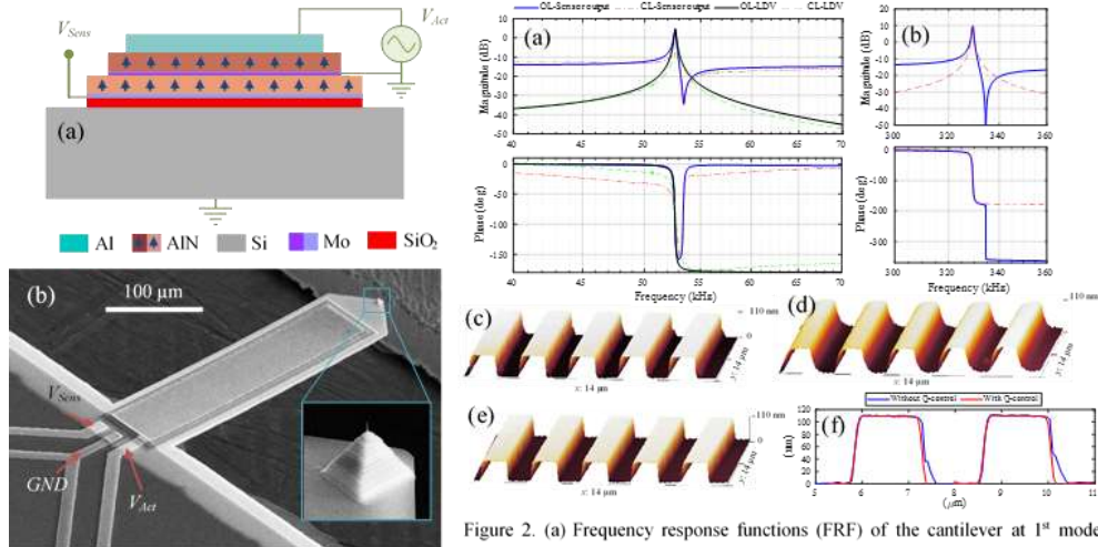
Figure 1. (a) Cross-sectional view and (b) SEM image of a microcantilever with a collocated piezoelectric actuator-sensor pair. The inset shows a Pt tip deposited with FIB/FEB.
