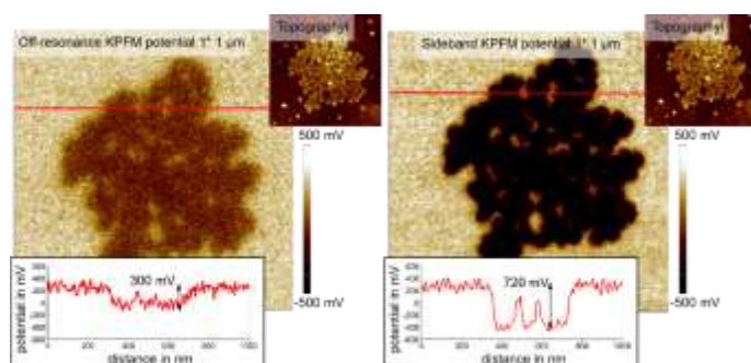
Figure 1: The same F14H20 aggregate was imaged using off-resonance and sideband KPFM. Cross sections (red) show improved lateral and potential resolution of sideband KPFM.
