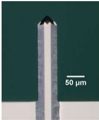
Figure 1: AFM cantilever used to test our model.
