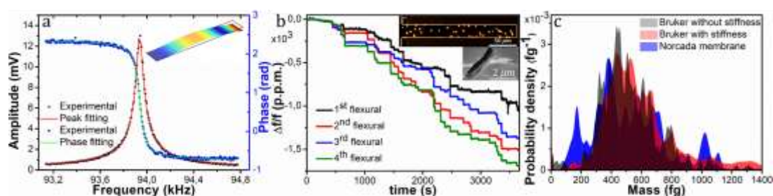
Fig. 1. (a) Fitting of the peak resonance and the phase of the second flexural mode (inset: FEM simulation) of the rectangular cantilever. (b) Relative frequency shift of the first four flexural modes of a microcantilever during the deposition of E. coli bacterial cells (inset: dark-field optical microscope image of the cantilever after the experiment with E. coli (top) and SEM image of a single bacterium (bottom)). (c) Probability density function of the E. coli mass for the NEMS used in this work.
