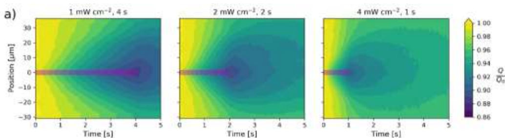
Figure 1: Thiolene conversion (represented as change in cantilever damping Q ) as a function of position relative to illumination and also duration of exposure. Reaction is found to occur tens of microns from the light source, and depends strongly on polymerization conditions and pattern size.
