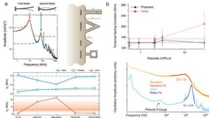
Fig 1: a) Calculation and comparison of the flexural spring constants from cantilever dynamics b) Comparison of torsional spring constant predictions derived with the proposed method and the Sader method in fluids of varying viscosity
