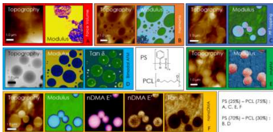
Figure 1. Typical maps of the mechanical properties of poly(styrene) - poly( \epsilon -caprolactone) polymer blends
