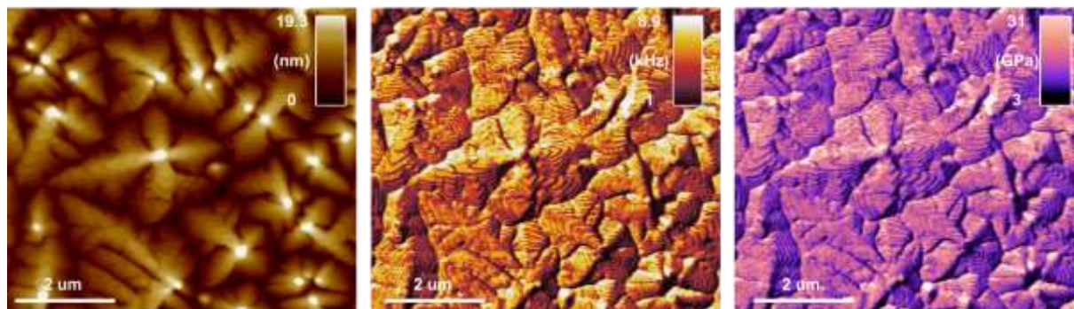
Figure 1. (a) Topography image of a 15 nm thick pentacene film. (b) Second mode frequency shift and (c) elastic modulus map.
