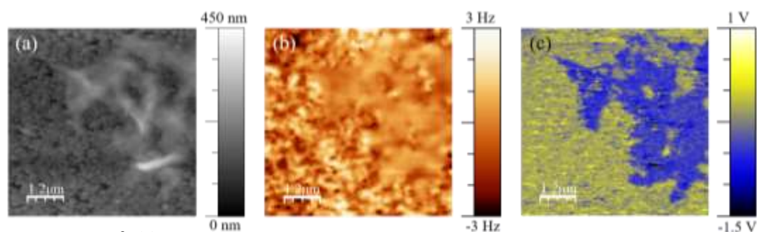
Figure 1. Images of (a) AFM, (b) MFM and (c) KPFM of an area where we distinguish uncovered nickel nanowires and a layer of PVDF-TrFE above them.
