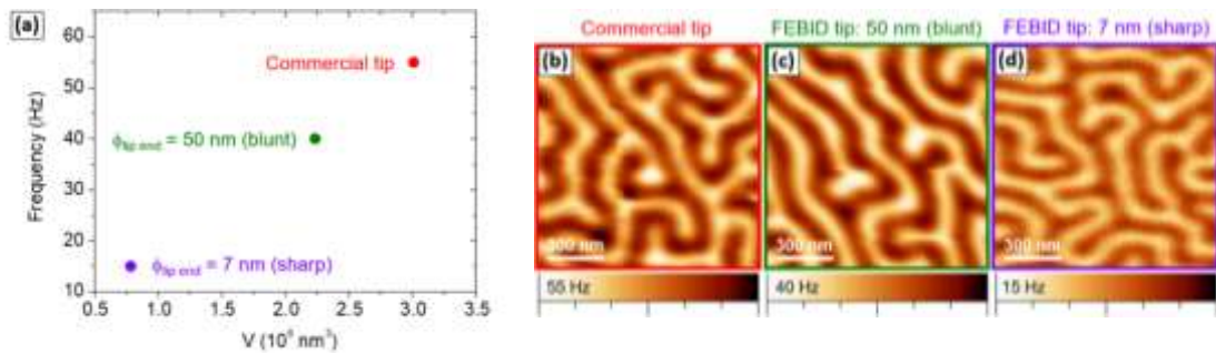
Figure1: Measurement of the frequency shift, related to the tip stray field, for three different probes, represented as a function of the magnetic tip volume. The corresponding MFM images, performed with (b) a standard commercial MFM probe (red), (c) a tip fabricated with an Fe-FEBID nanowire with a blunt tip end of 50 nm (green) and (d) a sharp tip end of 7 nm (purple), are shown.
