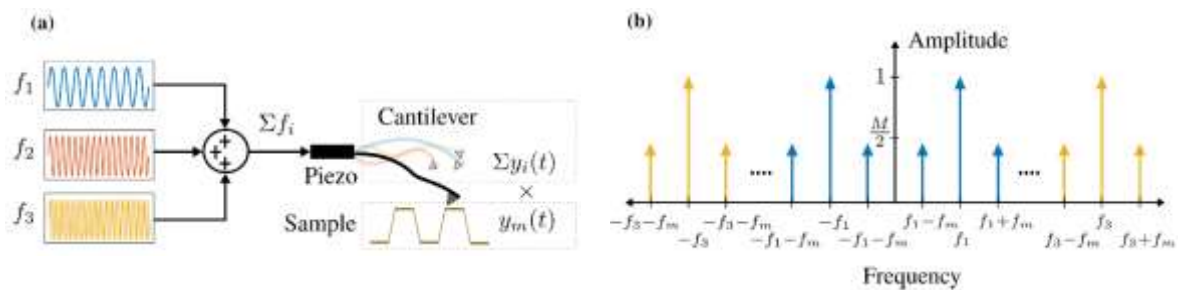
Figure 1: (a) Schematic diagram and (b) double-sided amplitude frequency spectrum of a cantilever oscillating at multiple frequencies amplitude modulated by a sample topography.
