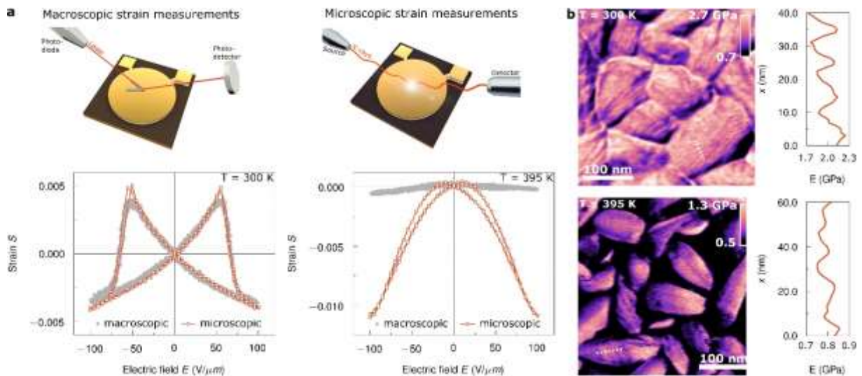
Fig. 1 Multi-scale characterisation of the ferroelectric polymer P(VDF-TrFE). a Macro- and microscopic electromechanical response of P(VDF-TrFE) in the ferro- and paraelectric states. b Nanomechanical maps of P(VDF-TrFE) in the ferro- and paraelectric states. The nanomechanical maps have been generated by bimodal AFM.
