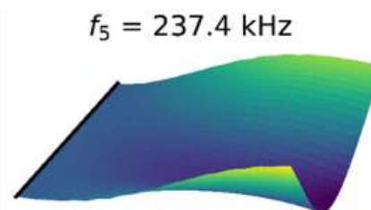
Figure 2: Simulated driven spectral response of the plate of figure 1 immersed in water.
