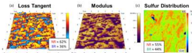
Figure 4. AFM nanomechanical analysis of a NR/BR blend showing (a) Loss Tangent image and (b) Modulus image. (c) NanoSIMS analysis of sulfur distribution in the blend. Images represent an area of 5 \times 5 \mu\text{m}^2 .
