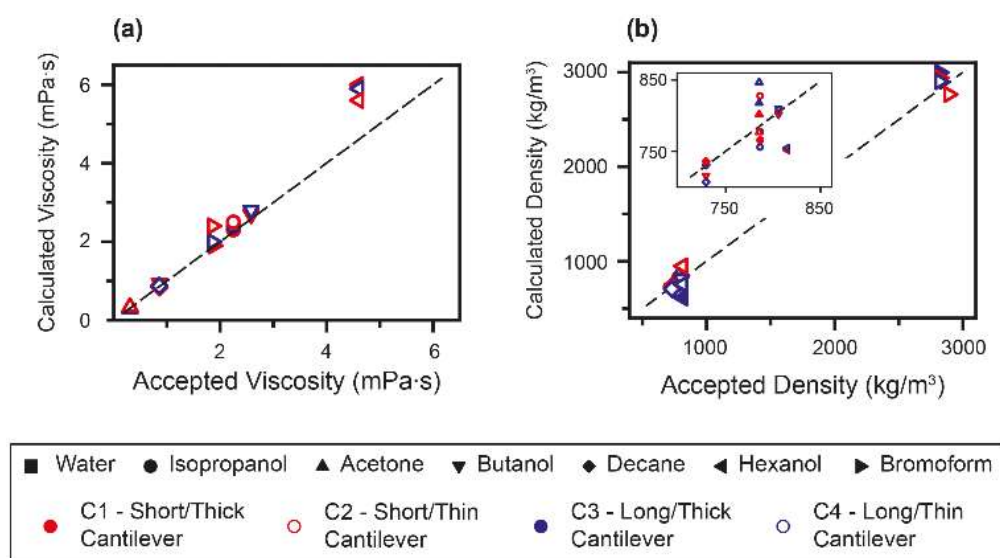
Fig 1: Comparison between the accepted and calculated viscosities (a) and densities (b) of the probed fluids. The modelled \eta and \rho compare well with the accepted values, as evidenced by their collapsing onto the line of unity gradient. The inset in (b) highlights the data points at lower densities [5].
