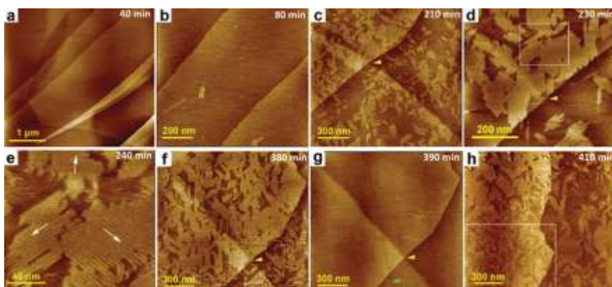
Fig. 1 AFM images of the evolution of the ordered structures at the water/graphite interface over time. All the images are acquired with the frequency-modulation AFM except for the one shown in (g), which is acquired with the tapping mode.
