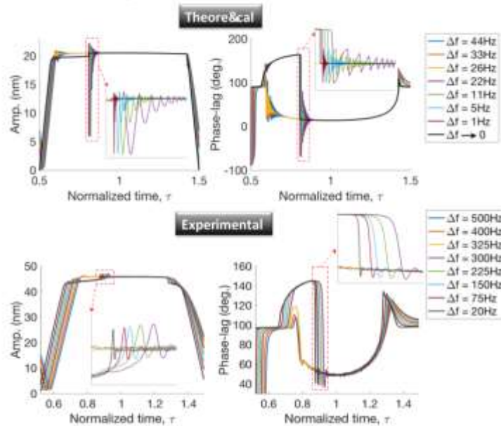
Fig. 2: Theoretical predictions and experimental results on rate dependent effects in ImAFM.
