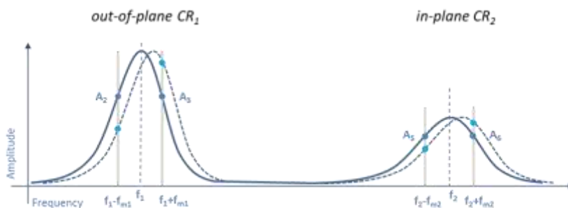
Figure 5: Frequency spectrum of cantilever in contact including the out-of-plane vertical resonance CR_1 and the in-plane lateral resonance CR_2 . The sidebands used for the resonance tracking ( A_2 and A_3 for the vertical resonance and A_5 and A_6 for the lateral resonance) are visualized in grey.
