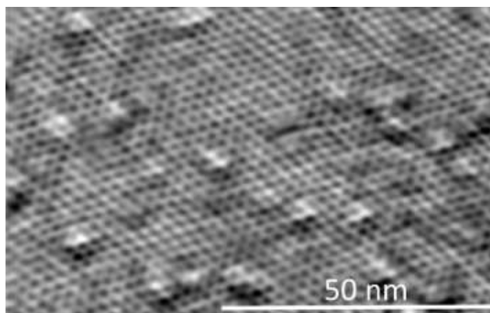
Fig. 1: nc-AFM frequency shift image of a 120×120nm 2 area of a 2D polymer. Parameters: f_{2nd} = 1\text{MHz} , A = 400\text{ pm} , \Delta f_{1st} = -27\text{ Hz} .
