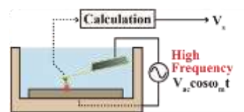
Fig. 1: (a) Experimental setup of OL-EPM
