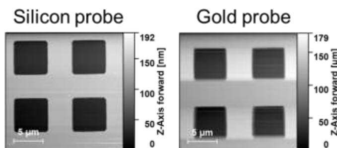
Fig 2. Comparison of LFM images obtained with commercial silicon probe and novel gold probe
