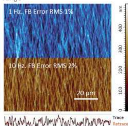
90×90×0,5 µm image of collagen fibers captured at 1 & 10Hz scanning rates in closed-loop mode
