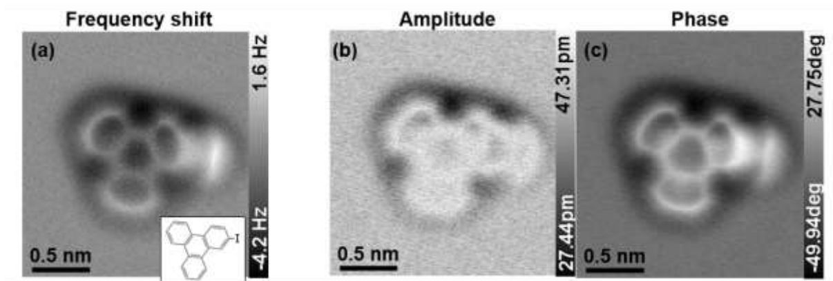
Figure 1: Constant height AFM images of 2-iodotriphenylene on Ag(111) imaged with a CO-functionalized tip in (a) frequency modulation and (b,c) Q-controlled amplitude modulation mode.
