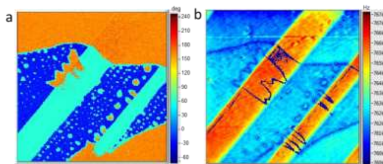
Figure 1 – a. Band Excitation PFM phase image and b. Band Excitation thermally excited CRF image of the a/c ferroelectric domains of a BTO single crystal
