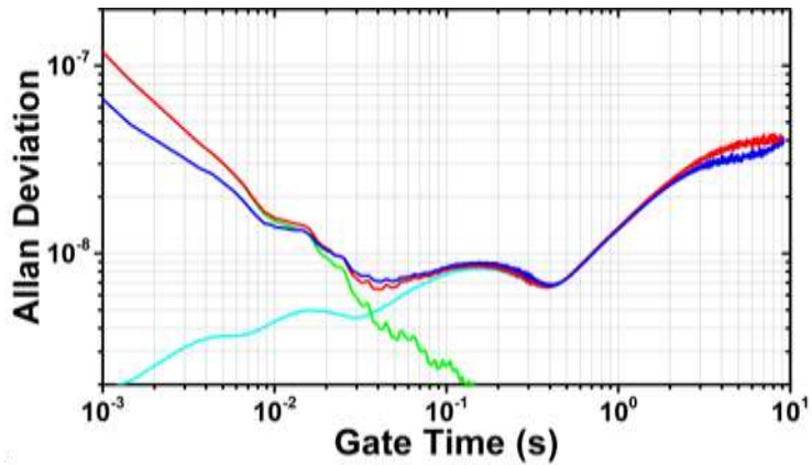
Figure 2: Frequency resolution obtained in closed-loop (blue) and calculated with our model from open-loop measurements (red). Cyan and green curves correspond to models previously used in the literature, only valid over a limited range of gate times.
