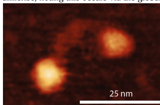
Figure 1: AFM reveals the structure of the protein NDP52
