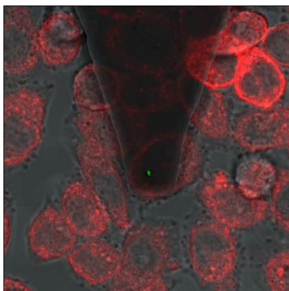
Figure. Combination of AFM and fluorescence microscopy image showing an AFM tip functionalized with a single virus while mapping virus binding sites on living mammalian cells
