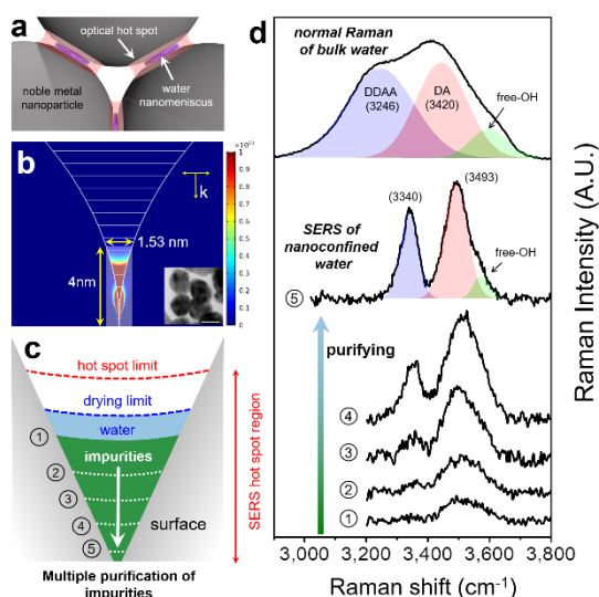
Fig. Surface enhanced Raman spectroscopy for ultra-purified nanoconfined water between gold particles.
