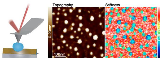
Fig. 1. Left) representation of the AFM nanomechanical mapping on vesicles adsorbed to the surface. Vesicles deform according to the affinity for the substrate. Middle) Topography image of DPPC:Chol (3:1, mol:mol) 50 nm extruded vesicles adsorbed on SiO 2 substrate in 150 mM KCl, 10 mM Tris, pH =7.4. Right) Its corresponding stiffness map.
