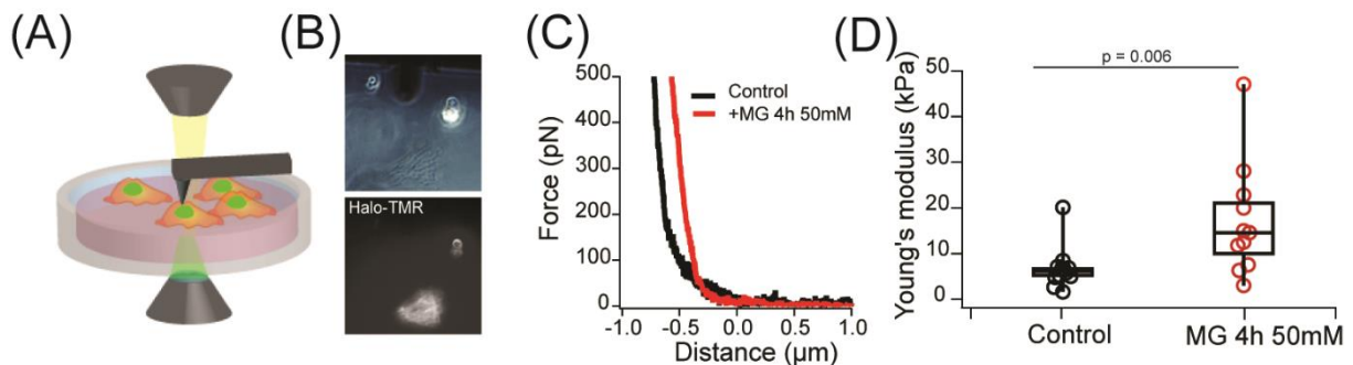
Figure 1. Methylglyoxal treatment induces cardiomyocyte stiffening. (A) Schematic cartoon of the experimental setup displaying a combined AFM-epifluorescence microscope. (B) Bright-field image of a skinned neonatal cardiomyocyte adhered on Matrigel (upper panel) and the corresponding fluorescence image showing titin labelled with Halo-TMR (bottom panel). (C) Examples of the approach segment of force-distance curves recorded on control (black trace) and skinned cardiomyocytes incubated with 50 mM MG for 4h at 37°C (red trace). (D) Young's modulus values of control and MG-treated skinned cardiomyocytes. Each dot represents the median value obtained for a single cell. Horizontal lines represent median values. Statistical significance calculated using the two sample Mann-Whitney U test.
