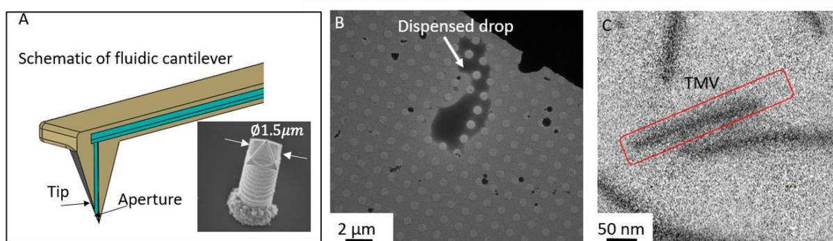
Figure 1: A blot-free cryo-microscopy sample preparation. (A) Schematic of the fluid-force microscopy probe. The inset shows a scanning electron microscopy image of the hollow cylindrical probe tip with a 1.5 μm diameter aperture. (B) cryo-EM image of vitrified 25 femtolitres of TMV solution on a quantifoil grid. (C) High-resolution cryo-EM image of the TMV virus from the dispensed sample.
