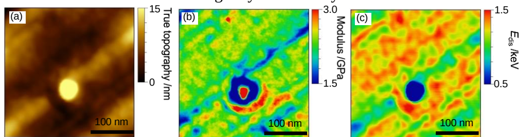
Figure 1: (a) True topography, (b) elastic modulus and (c) dissipated energy ( E_{dis} ) images captured surrounding a nanosilica in epoxy nanocomposites using AM-FM AFM method.
