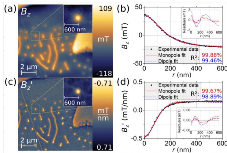
Figure: (a) B_z map of an [001] oriented MnNiGa crystallite. In the inset, a magnified image of an individual bubble domain is shown. (b) An angularly averaged B_z profile for the same bubble is shown together with point monopole and dipole fits. (c) and (d) present the same again but now based on B'_z data.
