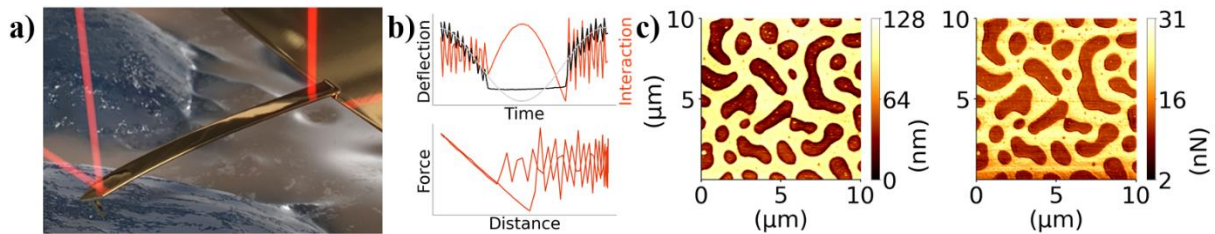
Figure 3: a) Artistic view of the laser configuration for photothermal off-resonance imaging. b) Photothermal off-resonance imaging signals acquired on a mica surface, captured as time-series data (above) and post-processed into force-distance representation (below). c) Topography (left) and adhesion map (right) of a PS-SBS block copolymer spin-coated on a mica surface acquired at 20 kHz excitation frequency with a comparable soft cantilever WM0.6 ( k = 0.6 N/m, f_0 = 350 kHz, Nanosurf).
