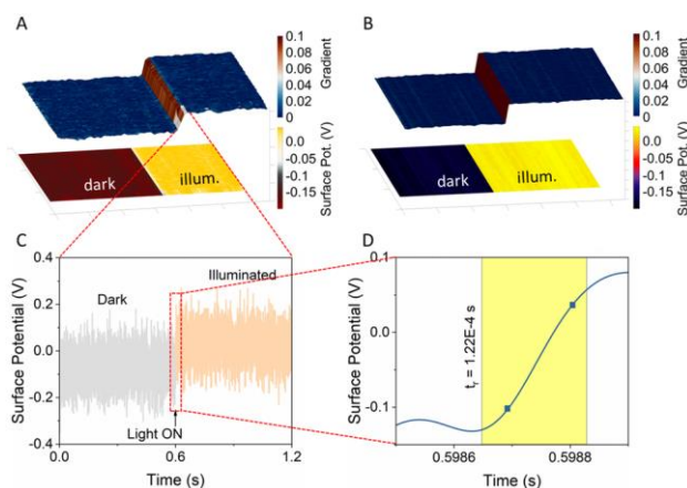
Fig. 1. Single-Pixel spectroscopic measurements on BiOI
