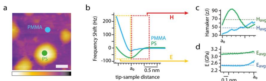
Fig. 1. Hamaker constant and Young's modulus derived from FM-AFM spectroscopy conducted at specific locations of a polymeric blend sample.
