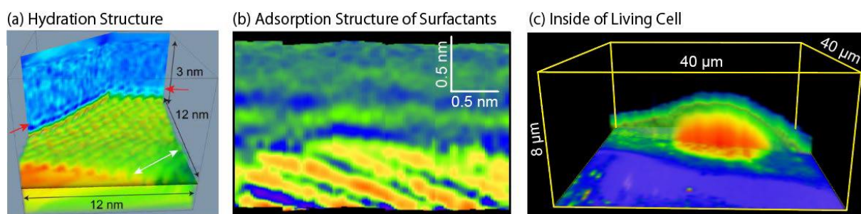
Fig. 1. 3D-AFM images of various 3D-SOSs. (a) Hydration structure formed on a cellulose nanocrystal (CNC) [1]. (b) Adsorption structure of surfactants (C16TABs) in its 10 ppm solution on the sapphire (0001) surface [2]. (c) Inside of live HeLa cell imaged at 37°C [3].
