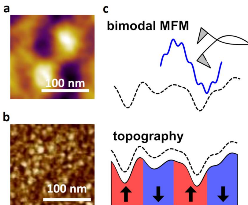
Figure: (a) High resolution image of the bimodal magnetic signal map AFM. interactions (b) Height profile of the surface. (c) Second pass scheme applied in bimodal AFM for imaging magnetic forces.
