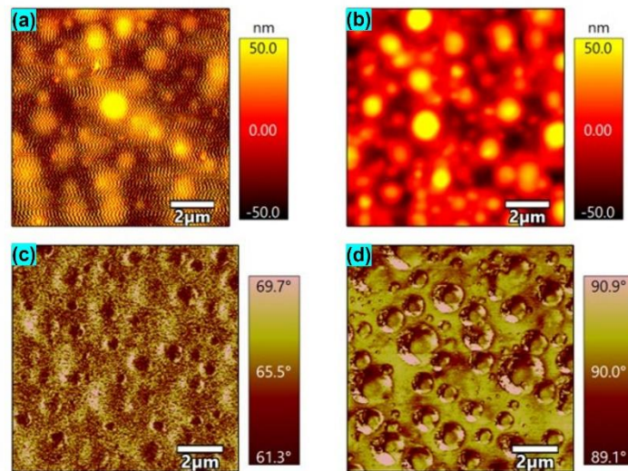
Figure 1. Topography images of (a) Nunano (b) Gold-modified Nunano from the fourth eigenmode and second-phase mapping of (c) Nunano (d) Gold-modified Nunano cantilevers from 1 st and 4 th eigenmodes of bimodal AFM.
