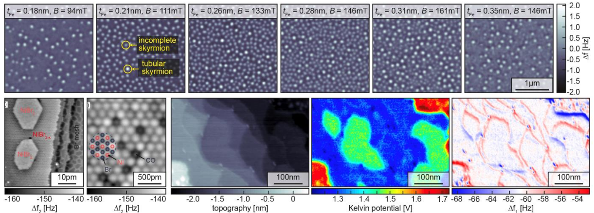
Figure 1: a) to f) MFM data of on F/Fi/F multilayers with different thicknesses t_{\text{Fe}} = 0.18 - 0.35 nm acquired with frequency-modulated tip-sample distance control revealing different densities of tubular/incomplete, i.e. two types of skyrmions. F = [\text{Ir}(1)/\text{Fe}(t_{\text{Fe}})/\text{Co}(0.6)/\text{Pt}(1)]_5 and \text{Fi} = [(\text{TbGd})(0.2)/\text{Co}(0.4)] \times 6/\text{TbGd}(0.2) . f) NiBr 2 islands on Au(111) showing NiBr 2 , NiBr 2-x , and Br-mesh phases. g) atomic resolution image of NiBr 2 . h), i), and j) topography, Kelvin signal, and MFM data acquired simultaneously using multifrequency techniques.
