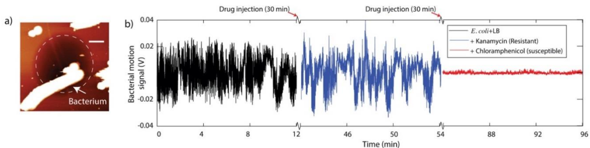
Fig. 1. (a) Atomic force microscope image of a graphene drum (shown by dashed circle) in the presence of single bacterium in liquid; (b) Motion of the drum with E. coli before and after adding Kanamycin (Resistant) and Chloramphenicol (Susceptible). White scale bar in Fig 1a is 4\mu\text{m} . In Fig 1b “LB” stands for Luria Bertani.
