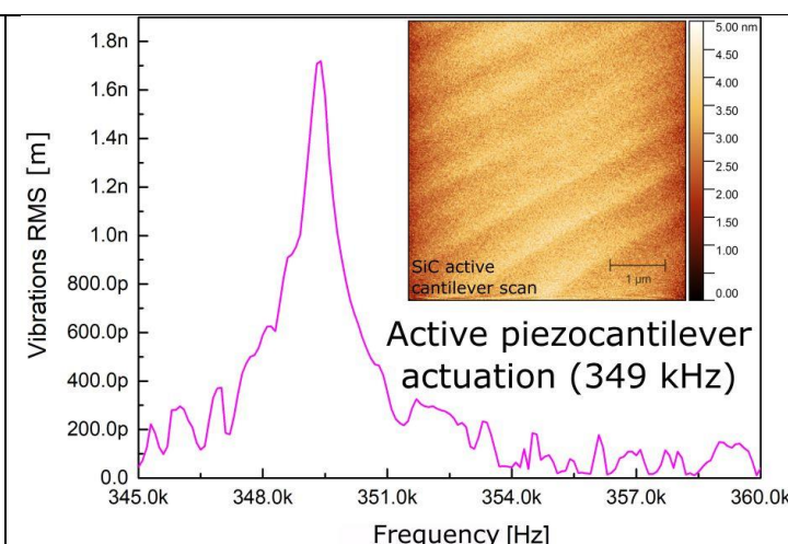
Fig. 2. Second eigenmode of the active piezoresistive cantilever and the topography of the silicon carbide surface recorded in the tapping mode
