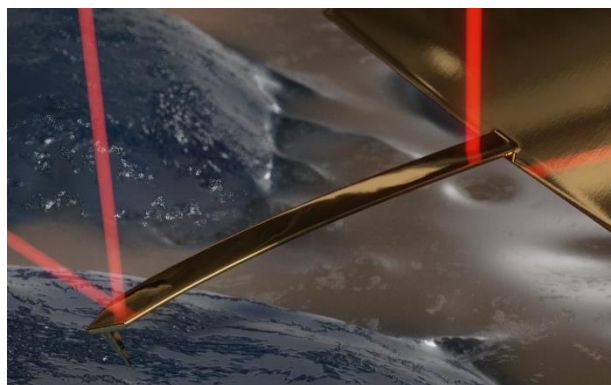
Figure 1: schematic representation of using photothermal actuation to directly actuate cantilever bending, through a second, intensity-modulated light source that is directed towards the base of the cantilever.
