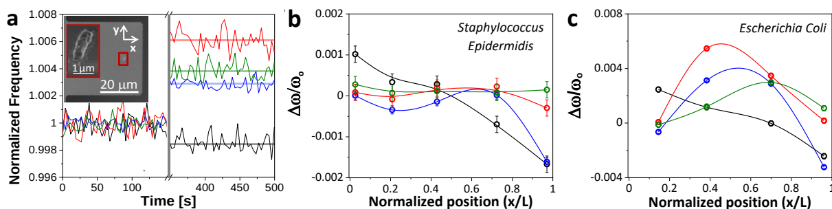
Figure 1. a. Normalized frequencies ( \omega/\omega_0 ) of the sensor 1 st flexural (black), 1 st torsional (red), 2 nd flexural (blue) and 2 nd torsional (green) before and after the adsorption of an Escherichia Coli cell. Insets show scanning electron microscope images of our sensor with the adsorbed bacteria cell. Solid lines indicate the averaged normalized frequencies after the bacterium adsorption. b-c. Relative frequency shift of the mechanical modes of the sensors induced by the adsorption of individual bacteria cells, respectively, versus the normalized longitudinal position (x-axis). All the cells are adsorbed on the sensors central position respect to the y-axis. Solid lines are guides to the eye.
