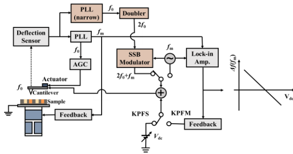
Figure 1: Block diagram of AFM and high—low KPFS. In the low KPFS, a signal V_{ac} \cos 2\pi f_m t is generated by the oscillator. In the high KPFS, a signal V_{ac} \cos 2\pi(2f_0 + f_m)t is generated by mixing the signal \cos 2\pi(2f_0)t and the signal \cos 2\pi f_m t in the SSB modulator.
