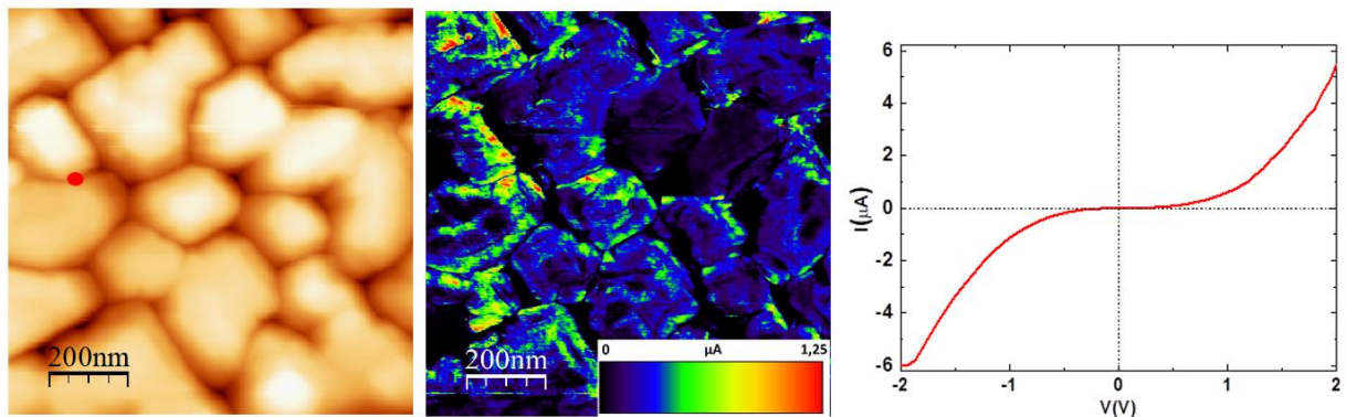
Figure: Topography (left) and current map (center) obtained by C-AFM in epitaxial (104) LCO/(100)SRO/(100)STO. IV curve (right) measured in the red dot on the topography image.
