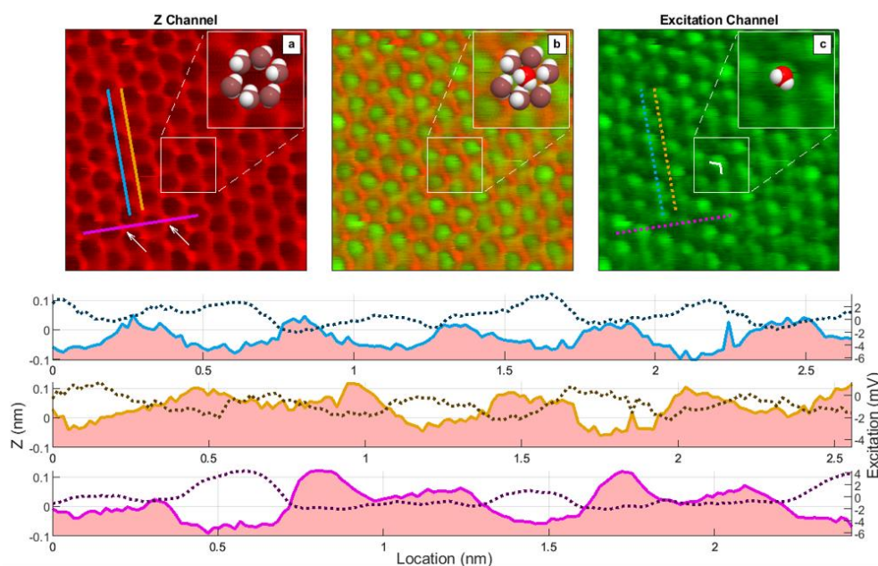
Figure 1: Extraction of hydration structure from a high-resolution scan of Muscovite mica surface immersed in a 100mM KCl and 1mM MgCl 2 solution. The top-left panel discloses the height map (Z-channel) plotted in red. The top-right panel depicts the corresponding excitation channel encoded in green. The top-center panel depicts superposition of the two signals. A clear overlap between bright excitation spots and Z-channel cavities is evident. The bottom series of three plots indicates one-dimensional profiles along the blue, yellow and purple lines. The Z and excitation signals are plotted using solid and dotted curves, respectively (also in the top panels). The two signals are evidently anti-correlated, indicating removal of a single water molecule from each cavity. The orientation of these molecules can be inferred from the non-circular shape of the bright spots in the excitation map (see white markings in inset c). As seen, the honeycomb pattern is made of six hydrating water molecules (inset a) adsorbed to the mica. Three of the water molecules are oriented slightly upwards (bright red spots), creating ~0.1 nm protrusions (see arrows along the purple line and the corresponding peaks in the bottom line-profile at 0.8 nm and 1.7 nm).
