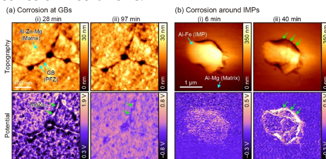
Figure 2: Topographic and potential images obtained by OL-EPM (a) at GBs and (b) around IMPs on the Al alloy surfaces.
