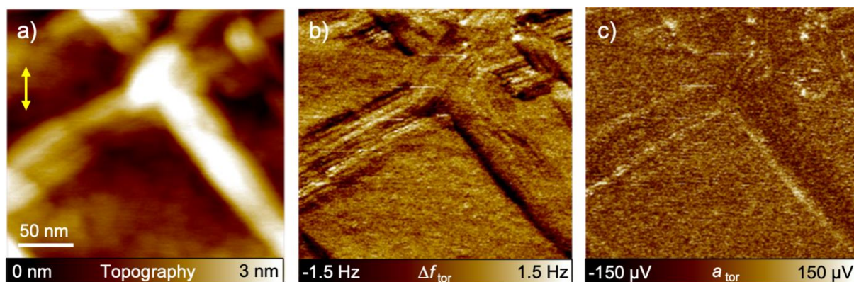
Fig. 1. Multifrequency AFM imaging of CNCs using the AMFlex-FMTor mode. a) Topography, b) torsional frequency shift and c) torsional drive amplitude images of two crystals crossing each other, thus representing different spatial orientations. The yellow arrow shows the direction of the shear motion of the AFM tip.
