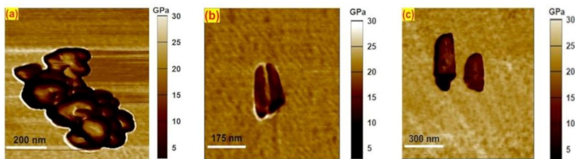
Figure 1. Young's modulus mapping of Cu-MOF (a) at room temperature, (b) at 300°C and (c) 500°C.
