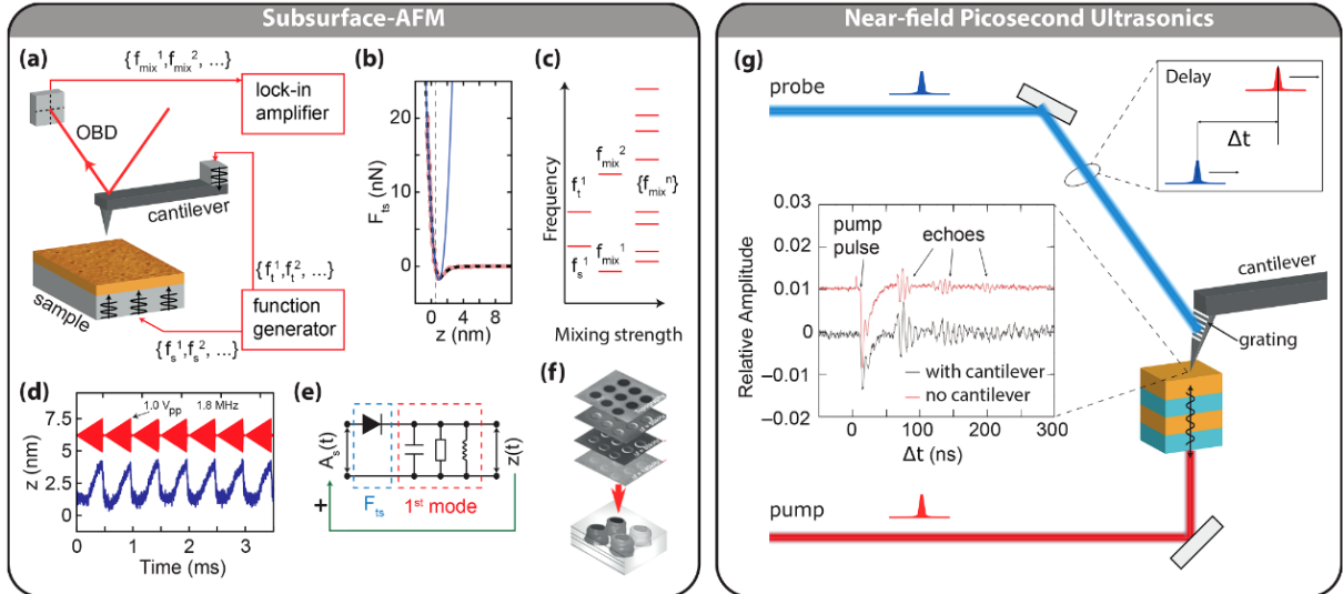
Figure 1. (a) Acoustic subsurface AFM uses one or multiple ultrasound excitations of the sample and/or cantilever and records the cantilever motion at their mixing frequencies using the optical beam deflection (OBD) method. These mixing frequencies are generated by the nonlinear tip-sample force F_{ts} , as depicted in (b) and (c). (d) UFM uses an amplitude modulated excitation signal on the sample (red). The cantilever only follows the modulation frequency, resulting in a rectifying effect (blue). (e) The cantilever response z(t) also modulates F_{ts} ; hence, it couples back into the F_{ts} (green arrow) complicating the modeling of the acoustic subsurface AFM. (f) By combining signals from different mixing frequencies, it is under certain conditions possible to reconstruct a 3D image of the measured device. (g) Near-field picosecond ultrasonics uses an ultrashort laser pump-probe technique in combination with a cantilever probe in order to perform pulse-echo measurements in the nanoscale (inset). By varying the delay \Delta t between the pump and probe pulse, the measurement depth can be controlled.
