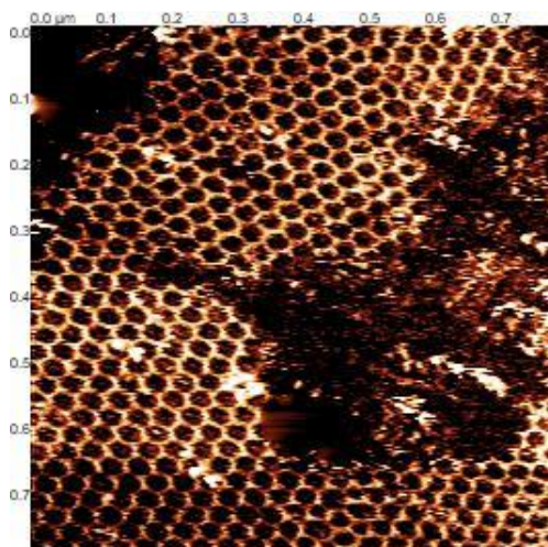
Figure 2: Assembly of blunt-end DNA tripods at steady state, acquired with HS-PORT AFM
