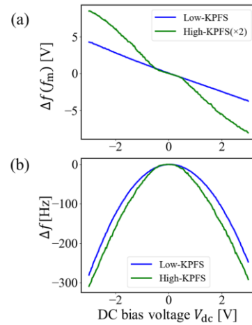
Figure 2: (a) \Delta f(f_m) - V_{dc} curves and (b) \Delta f - V_{dc} curves obtained on the n-type Si surface.
