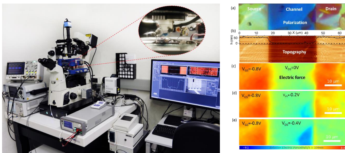
Left: Automated Multiparametric in-liquid SDM setup. Right: Polarization, topographic and electric force images at different applied voltages of the same region of an EGOFET.
