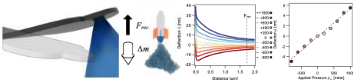
Figure 6 The principle of the hydrodynamic sensitivity, a cantilever is deflected by a recoil produced by ejecting masse from its aperture, similar to a classical rocket. From the linear dependency of the deflection on the applied pressure, the sensitivity is then calculated.
