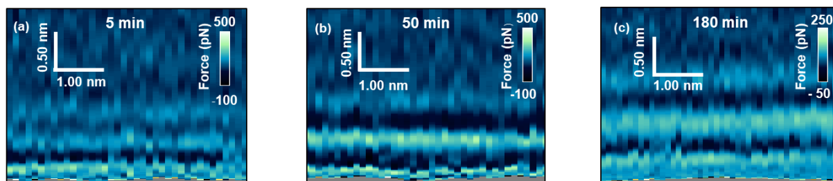
Figure 4. Time evolution of 2D force maps (x,z) of graphite-water interfaces extracted from 3D AFM volume images.
