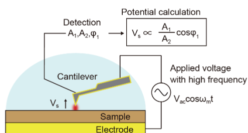
Figure 1: OL-EPM setup.
