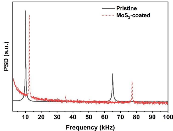
Figure 1. Thermal noise spectra of pristine and MoS 2 - coated cantilevers.
