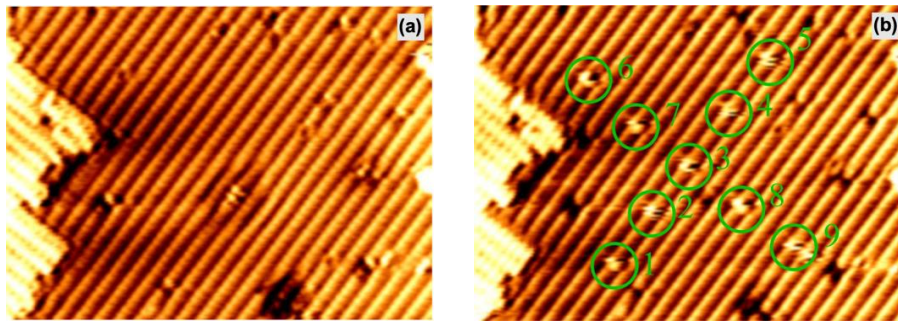
Figure 1. Atomic precision lithography on hydrogen passivated silicon
