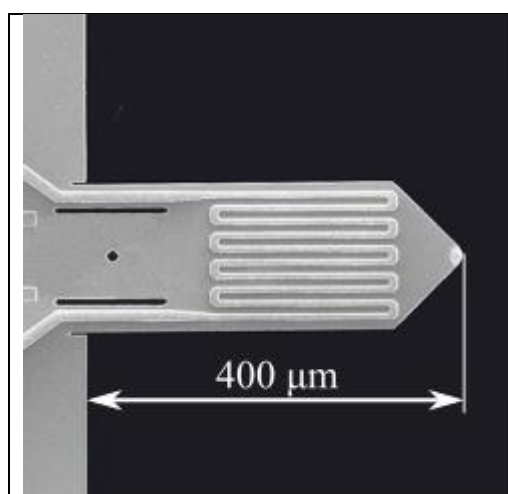
Fig. 1. Active piezoresistive cantilever ( https://www.nanoanalytik.net )
