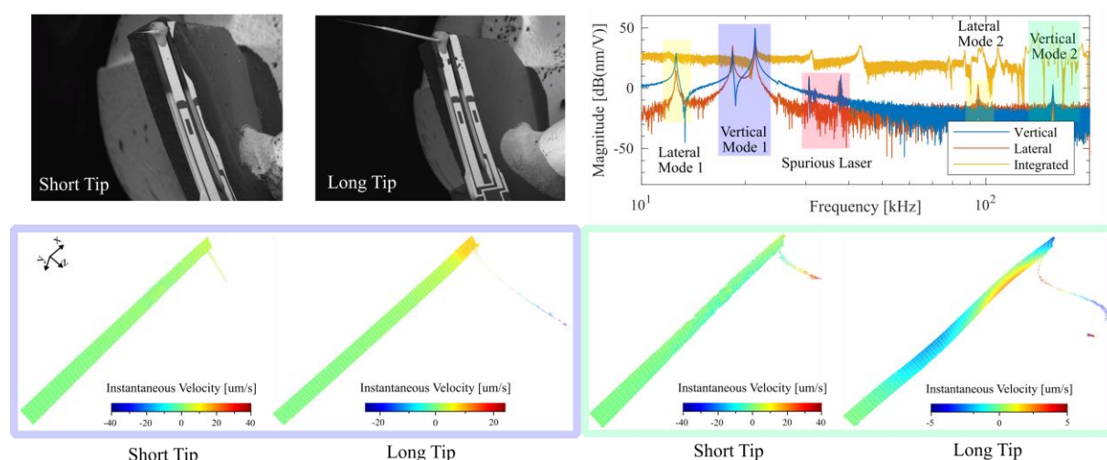
Figure: Top row: SEM images of two of the experimentally investigated qPlus sensors and frequency response of the long tip qPlus sensor measured with a laser Doppler vibrometer (MSA-100 3D) from the top (vertical) and side (lateral) and using an integrated current amplifier (integrated). Bottom row: Lateral deflection mode shapes of the short and long tip qPlus sensor prong and tip at the first and second vertical mode (color coded according to the frequency response). Significant lateral tip vibrations can be observed at the first and second vertical mode.
