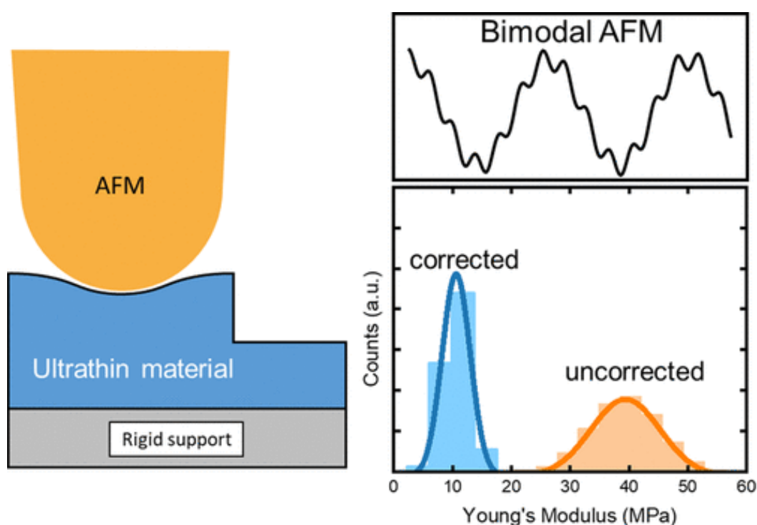
Figure - Scheme of a tip, ultrathin-layer and solid support interface. The bimodal AFM measurement of the nanomechanical properties of such a system yields an overestimation of the Young's modulus due to the bottom effect. With the bottom effect correction, the corrected value of the Young's modulus is measured.
