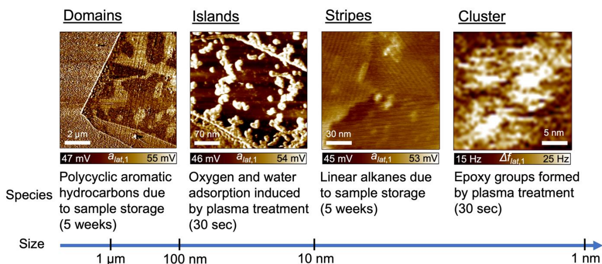
Figure 1: Different adsorbate structures visualized by multifrequency atomic force microscopy that were formed upon ambient storage and oxygen-plasma treatment of multilayer graphene. The three first images show the drive amplitude for the first lateral cantilever eigenmode to maintain the oscillation amplitude and the last one shows the lateral frequency shift of the first lateral eigenmode.
