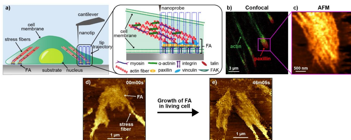
Fig. 1: (a) Schematic of 3D nanoendoscopy measurement of FAs. (b) Confocal image of actin stress fibers connected to FAs (paxillin and actin staining) and (c) a corresponding AFM image of an individual highlighted FA. (d) and (e) represent contact point mapping images of the same FA at 0 and 46 minutes of imaging, indicating the maturation of the FA.
