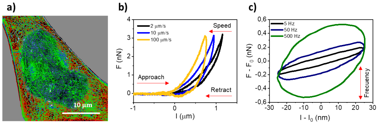
a) AFM nanomechanical map. b) Force-distance curve (nanoindentation) on a HeLa cell at different velocities. c) Oscillatory force-distance curves (nanorheology) on a HeLa cell at different frequencies.
