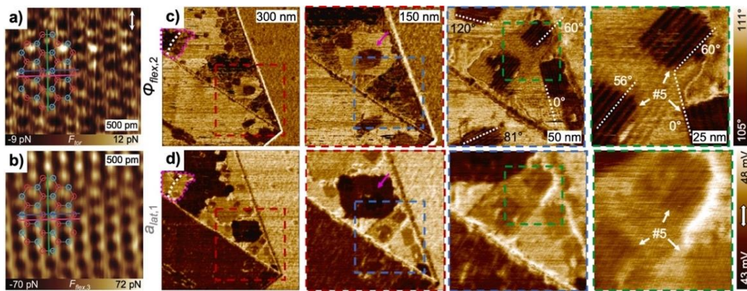
Figure 1: Trimodal AFM imaging of HOPG and adsorbates on few-layer graphene/graphite. a) Force deconvolution for in-plane and b) out-of-plane tip-sample interactions. c) Out-of-plane and d) in-plane tip-adsorbate interactions on different length scales. The surface reflects partially a graphene flake with two distinct layer thicknesses (left portion of the first images) on SiO 2 (right portion).
