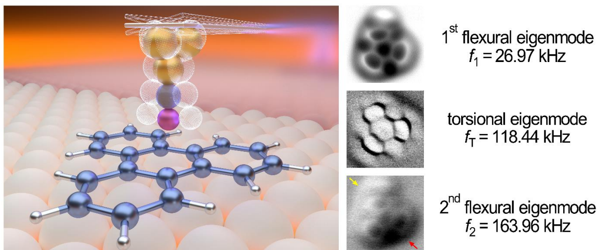
Figure: Using the torsional eigenmode and the 2 nd flexural eigenmode of a qPlus sensor for bond imaging AFM with CO functionalized tips at low temperatures in ultrahigh vacuum. When the torsional eigenmode is excited the tip oscillates nearly parallel to the surface (see left scheme). This is useful for performing lateral force microscopy with single chemical bond resolution (see AFM image in the right middle).
